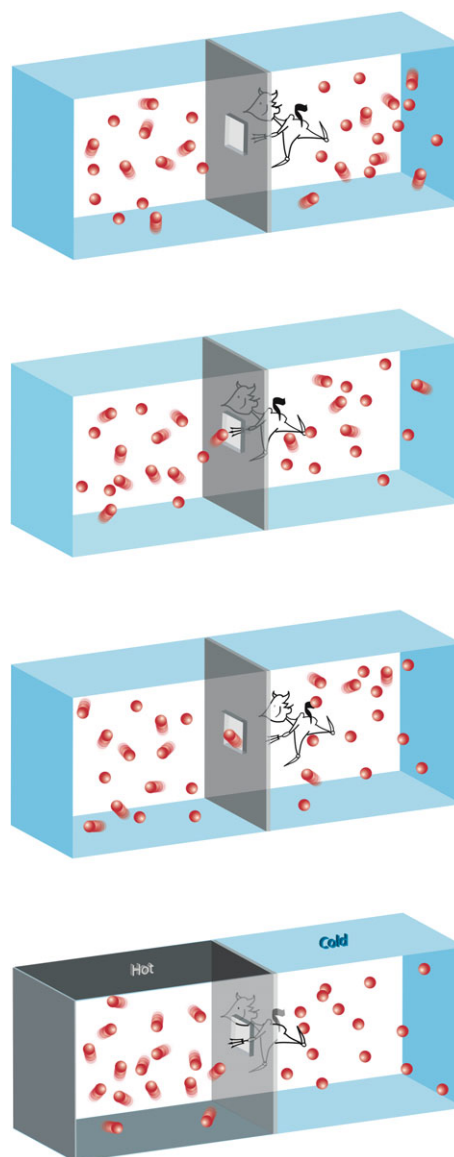
Fig. 2. The original Maxwell's demon. The molecules in a vessel full of gas at uniform temperature are moving with highly variable velocities, though the mean velocity of any great number of them, arbitrarily selected, is almost exactly uniform. Now, let us suppose that such a vessel is divided into two compartments, left and right, by a division in which there is a small hole, and that a demon, who can see the individual molecules, opens and closes this hole, so as to allow only the swifter molecules to pass from right to left, and only the slower ones to pass from left to right. It will thus, without expenditure of work, raise the temperature of the left compartment and lower that of the right compartment, in apparent contradiction to the second law of thermodynamics.
