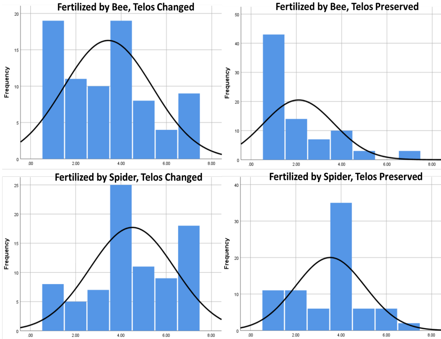
Figure 4: Distributions in Offspring Judgments for Telos Changed and Preserved
