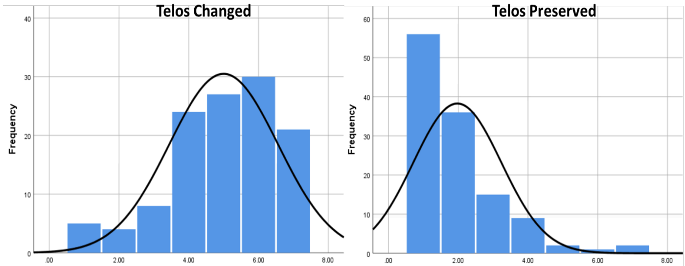
Figure 2: Distributions in Categorization Judgments for Telos Changed and Preserved
