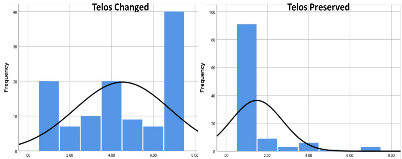
Figure 3: Distributions in Categorization Judgments for Telos Changed and Preserved
