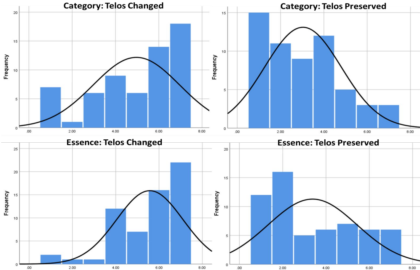
Figure 5: Distributions in Categorization and Essence Judgments for Telos Changed and Preserved
