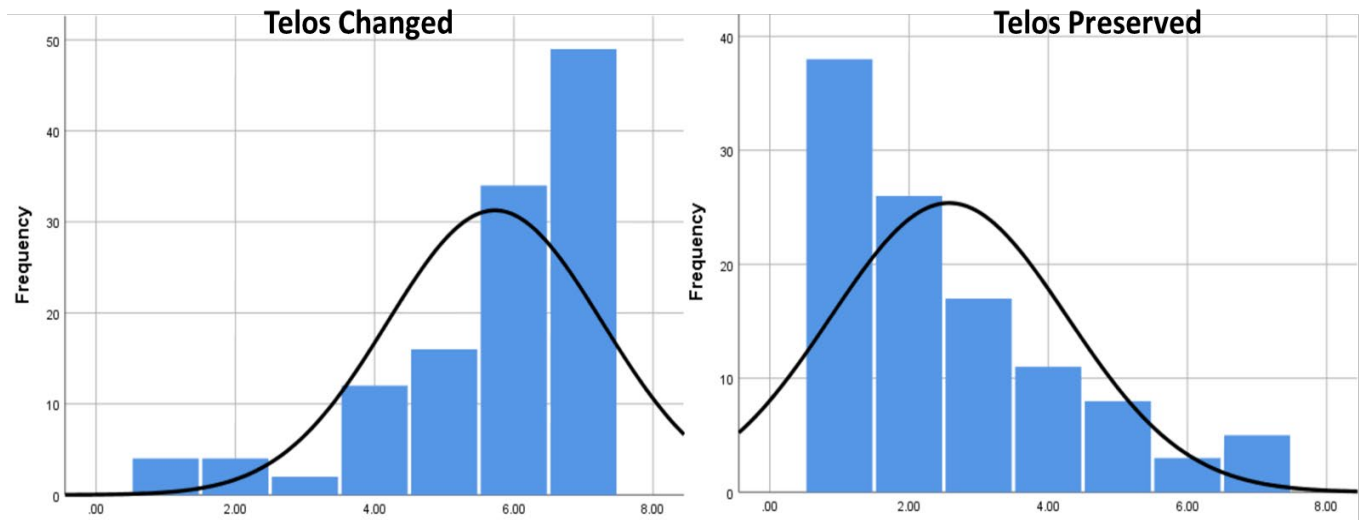
Figure 1: Distributions in Categorization Judgments for Telos Changed and Preserved
