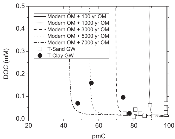
Fig. 8. ^{14}\text{C} -TOC groundwater from T-Sand (open squares) and T-Clay (filled circles) and the modelled evolution in the age of bulk DOC through the mixing of sedimentary OM and modern OM (Lawson et al., 2013). Measured ^{14}\text{C} -TOC concentrations are compared with model concentrations of DOC calculated based on two-component mixing of 0.002 mM of modern OM with sedimentary OM with ages of 100, 1000, 3000, 5000 and 7000 years. Mixing profiles demonstrate the requirement for contributions of modern DOC and place upper limits on the age of sedimentary OM contributions of 7000 years. The analytical uncertainties in pmC lie within the symbol shown.
