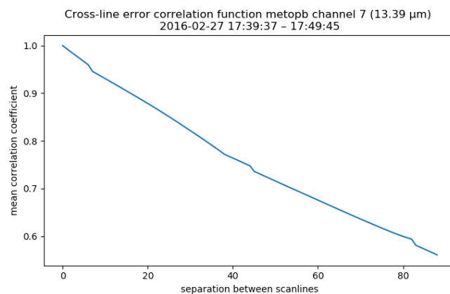
Figure 4. Cross-line error correlation function representative of error correlations from structured effects for the data in Figure 1.
