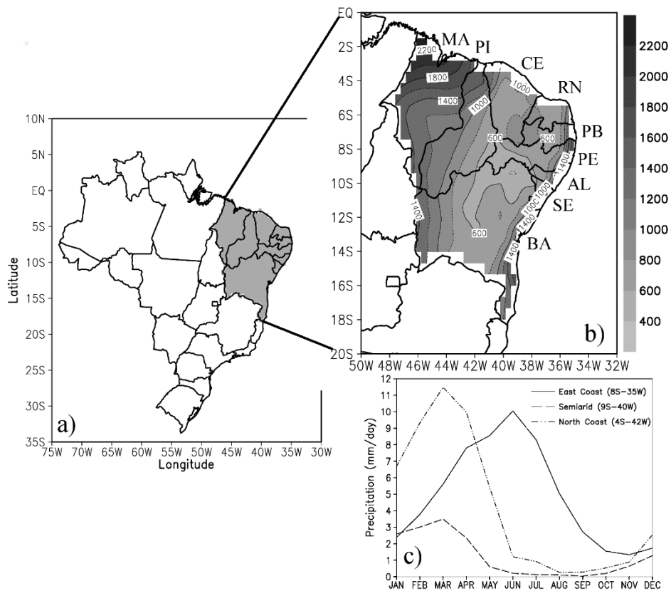
Fig. 1 Northeast Brazil geographical location and study area (a) and annual (b) and monthly (c) precipitation climatology.
