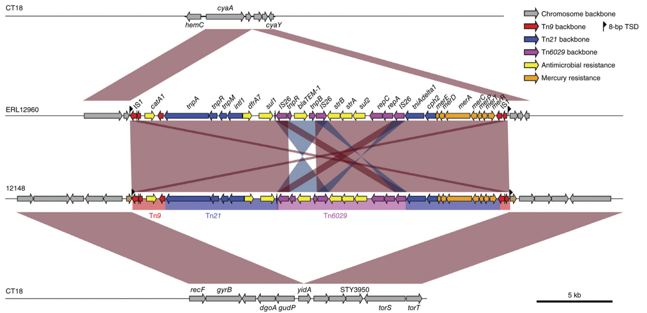
Figure 5. Insertion site of the 24-kb composite transposon in CT18. A comparative analysis using genoPlotr 48 of CT18 and H58 isolates ERL12960 (ERR343327) and 12148 (ERR343322) showed two integration sites of the transposon in the chromosome. The nucleotide sequence of the composite transposon was identical to that in the IncHI1-PST6 plasmid of H58 isolate 10425_1_48_Viety3-193_1997, which was sequenced for comparison. Tn, transposon; TSD, target site duplication.
