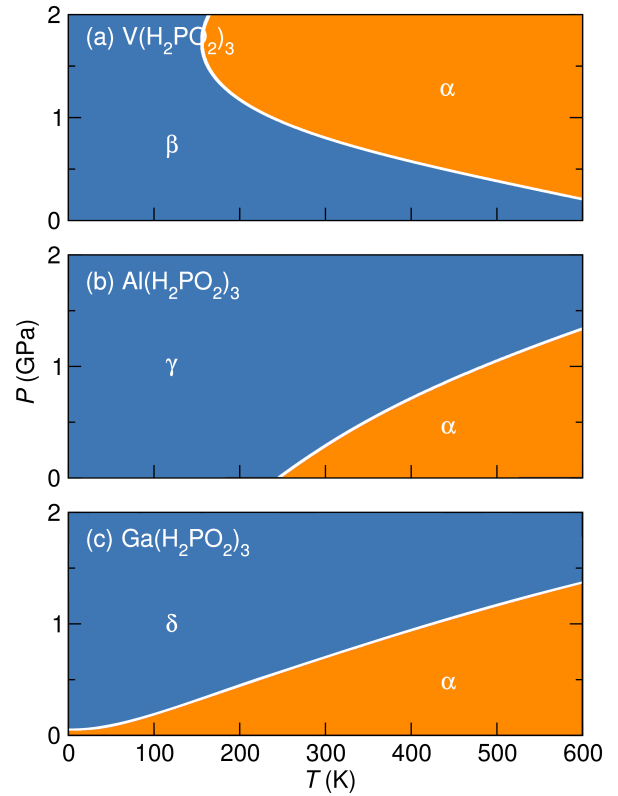
Fig. 3 Calculated P - T phase diagrams for each metal system, and the two observed polymorphs seen each in each. (a) V system, \alpha - \beta polymorphs. (b) Al system, \alpha - \gamma polymorphs. (c) Ga system, \alpha - \delta polymorphs.
