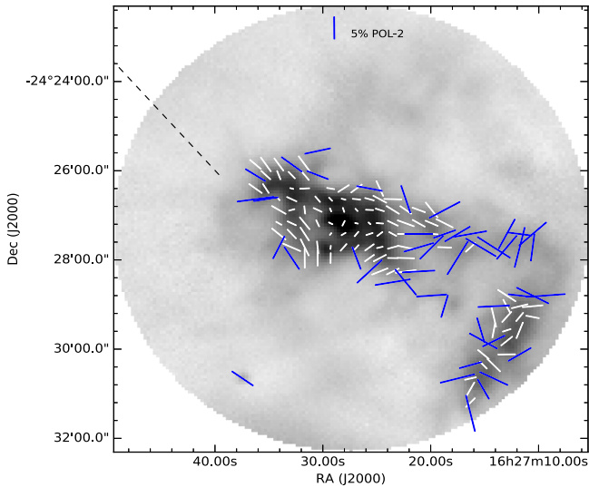
Figure 4. Smoothed B -field orientations in Oph-B, shown on the 850 \mu\text{m} dust emission map from SCUBA-2. The polarization data are averaged over 4 pixels (an effective pixel size of 8'' using 2 \times 2 binning). White vectors correspond to data with P < 5\% , while blue vectors correspond to data with P > 5\% . The vectors are selected to have PI/\delta PI > 2 and are rotated by 90^\circ to show the inferred B -field morphology. A reference vector with 5% polarization is given for scale. The black dashed line shows the orientation of the Galactic Plane at the latitude of the cloud.
