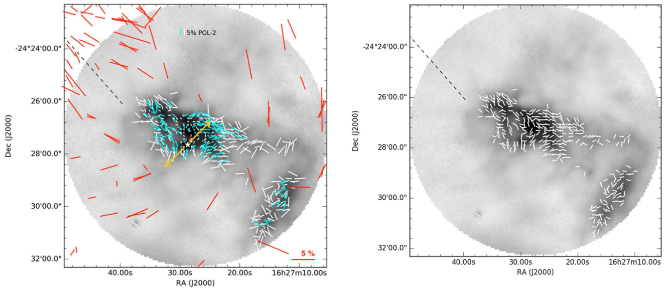
Figure 3. Left panel: B -field orientation in Oph-B from 850 \mu\text{m} dust polarization data. The background image shows the dust continuum map at 850 \mu\text{m} from SCUBA-2. The white and cyan color vectors correspond to data with PI/\delta PI > 2 and PI/\delta PI > 3 , respectively. The vectors are rotated by 90^\circ to show the inferred B -field morphology. The white star symbol represents the position of IRS47, with its associated bipolar outflow shown using a double-headed arrow in yellow. A 5% polarization vector is shown for reference. The red vectors show the B -fields mapped using deep NIR observations by Kwon et al. (2015). The black dashed line shows the orientation of the Galactic Plane at the latitude of the cloud. Right panel: same as left panel (except NIR data), but the vectors are of uniform length, rather than scaled with polarization fraction.
