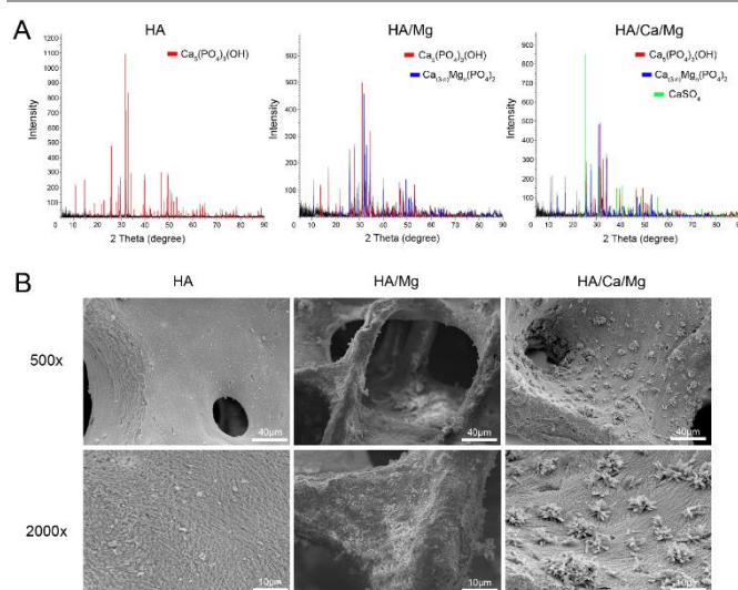
Fig 1. Composition and surface characteristics of different scaffolds. (A) X-ray diffraction of scaffolds. (B) SEM images of the surface morphology of scaffolds.
