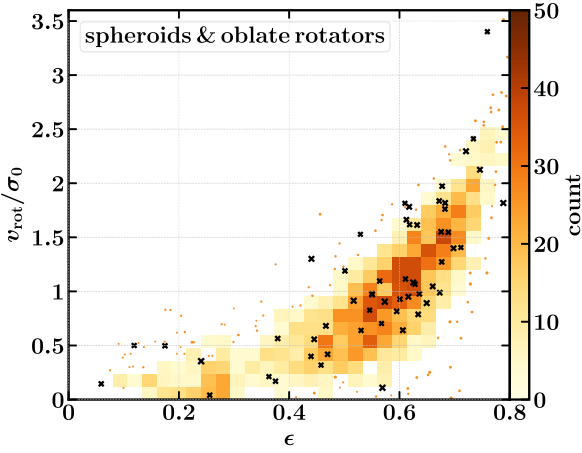
Figure A1. The relationship between v_{\text{rot}}/\sigma_0 and flattening, \epsilon , for galaxies with M_* > 10^{9.5} M_\odot and which are (i) spheroidal ( \epsilon < 0.3 ) or (ii) oblate ( T < 1/3 ) galaxies and have their morphological and rotational axes aligned to within 10^\circ . The two-dimensional histogram and orange dots represent the 2703 galaxies of Ref-L100N1504 that satisfy these criteria (as per the bottom panel of Fig. 4), whilst black crosses denote the corresponding 57 galaxies from Recal-L025N0752. Visual inspection suggests that the weak convergence behaviour of v_{\text{rot}}/\sigma_0 and \epsilon is good, an impression corroborated by the two-sample Kolmogorov–Smirnov test in each case.
