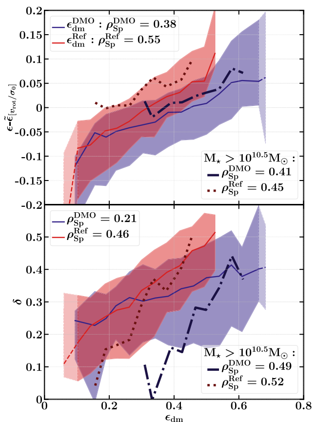
Figure 7. The deviation of a galaxy’s flattening, \epsilon from the median flattening for galaxies of similar v_{\text{rot}}/\sigma_0 ( \epsilon - \bar{\epsilon}_{[v_{\text{rot}}/\sigma_0]} , upper panel), and the anisotropy of the stellar velocity dispersion ( \delta , lower panel), as a function of the flattening of the inner dark matter halo, \epsilon_{\text{dm}} . The solid lines and shaded regions denote the median relations and the 1\sigma (16th–84th percentile) scatter about them, respectively. The red curves adopt \epsilon_{\text{dm}}^{\text{Ref}} as the halo flattening diagnostic, the blue curves adopt \epsilon_{\text{dm}}^{\text{DMO}} . Medians are drawn with dashed lines in bins sampled by fewer than five galaxies. Dotted and dot-dashed thick lines represent the corresponding median relations for the high-mass ( M_* > 10^{10.5} M_\odot ) sub-population for which only bins sampled by more than five galaxies are drawn.
