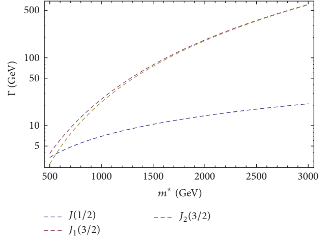
FIGURE 1: Total decay width of excited neutrinos according to their mass. Here, it is taken as \Lambda = m^* and f = -f' = 1 for excited spin-1/2 neutrinos and c_V = c_A = 0.5 ( i = 1, 2 ) for excited spin-3/2 neutrinos for the two phenomenological currents.
