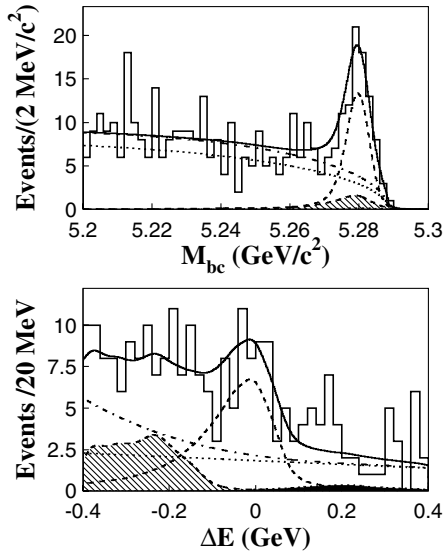
FIG. 1. The upper plot is the M_{bc} projection for events in the \Delta E signal region -0.20 \text{ GeV} < \Delta E < 0.07 \text{ GeV} ; the lower plot is the \Delta E projection for events in the M_{bc} signal region 5.27 \text{ GeV}/c^2 < M_{bc} < 5.29 \text{ GeV}/c^2 . The solid curve shows the results of the fit. The signal component is shown as a dashed line. The continuum background is shown as a dotted line. The sum of b \rightarrow c and continuum components is shown as a dot-dashed line. The hatched (dark) histogram represents the B^0 \rightarrow \rho^+ \rho^- ( B^0 \rightarrow \pi^0 \pi^0 ) background.
