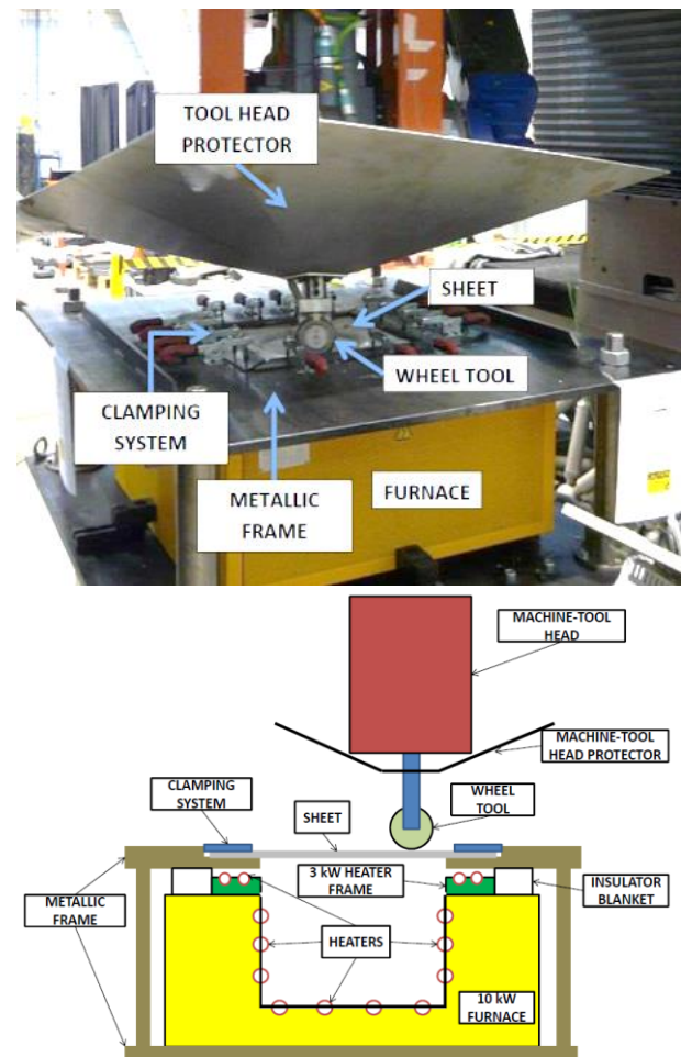
Fig. 1 Hot SPIF equipment used for the trials
