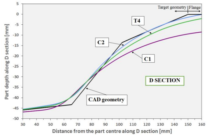
Fig. 20 Shape profiles of a wall with low (15°) and high (38°) angle (D section) extracted from the deviation maps of Fig. 18
