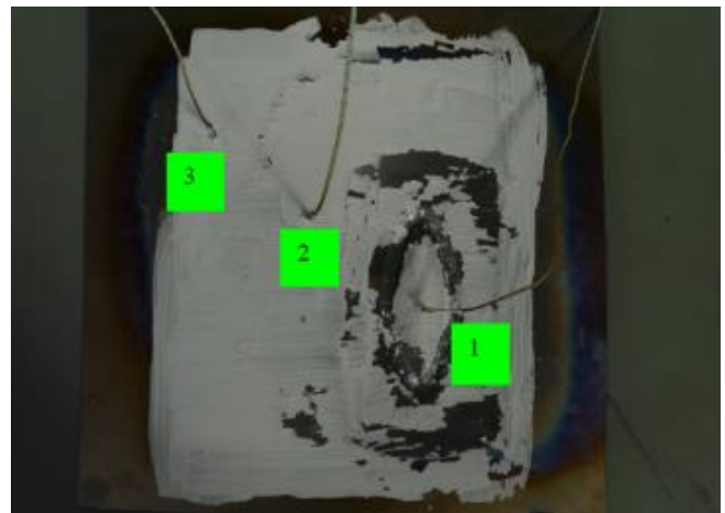
Fig. 3 Sheet coated with Boron Nitride for emissivity calibration trial
