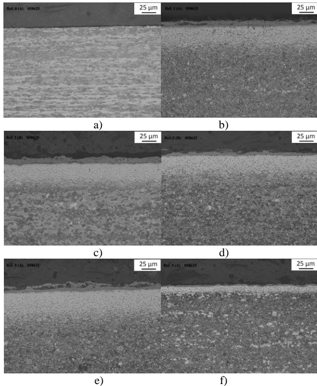
Fig. 22 Microstructure of Ti-6Al-4V: a) As-received, Ref.0 / b) Ref.1, c) Ref.2, d) Ref.3, e) Ref.4 and f) Ref.5 extracted from a previously heated and formed sample (400x magn.)
