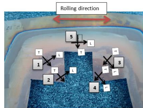
1 to 5 specimens extracted from the processed part
