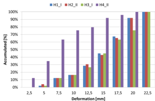
Fig. 11 Cumulative deviation histograms of the sheets after heating trials of H1, H2, H3 and H4
