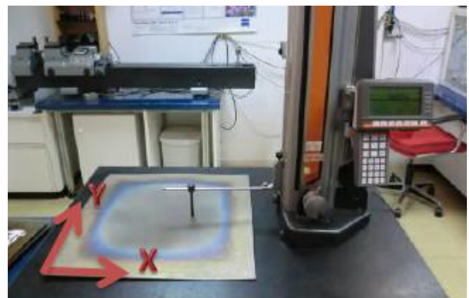
Fig. 4 Table of flatness to measure the non-deformed sheets
