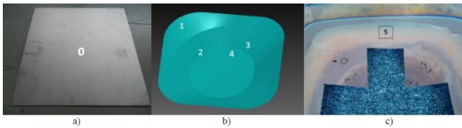
Fig. 6 Location of the specimens for metallographic analysis a) 0 position on the as-received Ti-6Al-4V blank, b) 1, 2, 3 and 4 positions located on the 3D CAD geometry and c) 1, 2, 3, 4 and 5 positions on the C2 sample
