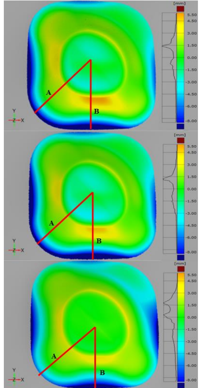
Fig. 15 Colour map of deviations for T2 (above), T3 (middle) and T4 (below) trials.
