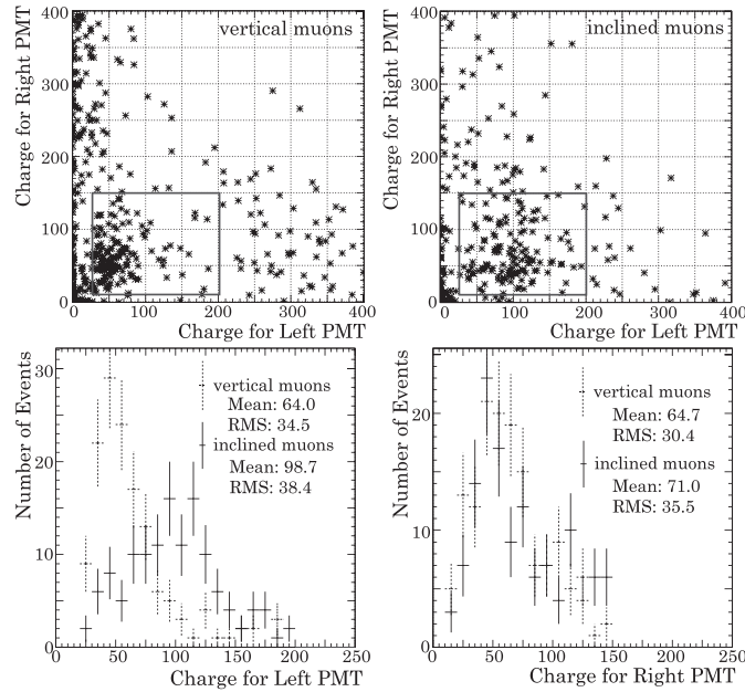
Figure 8. Top panel shows that the correlation of charge between Left and Right PMT in case of both vertical (left side) and inclined (right side) muons. Bottom panel shows the charge distribution of Left PMT (left side) and Right PMT (right) using events located in box of above panel in case of vertical (dotted line) and inclined (solid line) muons. Obviously the charge of Left PMT was increased in case of vertical muons.
