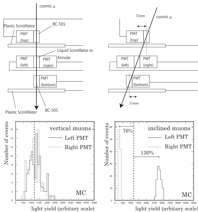
Figure 4. Top panel shows that the setup of the measurement of pulse shape using vertical (left ) and inclined (right) muons. The bottom panel shows that the expected charge distribution for Left (solid line) and Right (dotted line) PMT, respectively. The averaged charge is almost same for left and right PMT in case of vertical muons. On the other hands, the charge for Left PMT moved about 130% but the charge for Right PMT was decreased about 76%. This is due to the directionality of Cherenkov lights.
