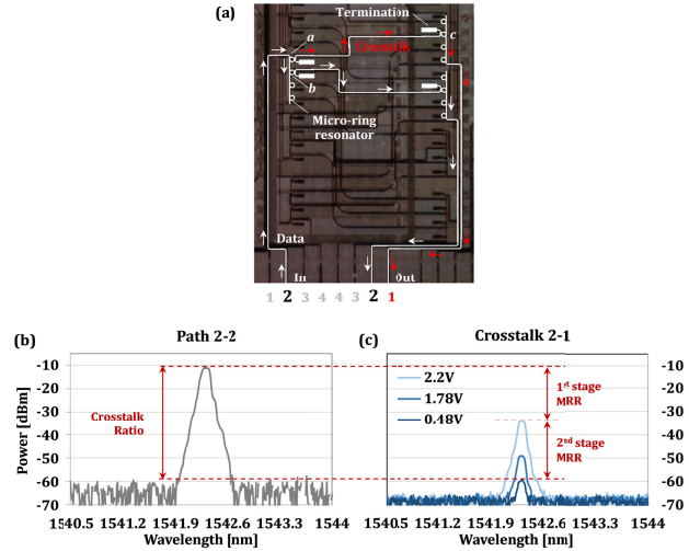
Fig. 8. Crosstalk breakdown measurement. (a) Outlined optical paths under test: data routed in path 2-2 and the crosstalk leakage to output 1 (crosstalk 2-1). Measured power spectrum for (b) the data at output 2 and (c) crosstalk leakage at output 1 with thermal tuning on the 2 nd stage output MRR to minimize the crosstalk leakage.
