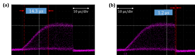
Fig. 11. Measured optical time-domain response of the thermo-optic switch. The cursors show the 10% to 90% power points for (a) the rise edge and (b) the fall edge.
