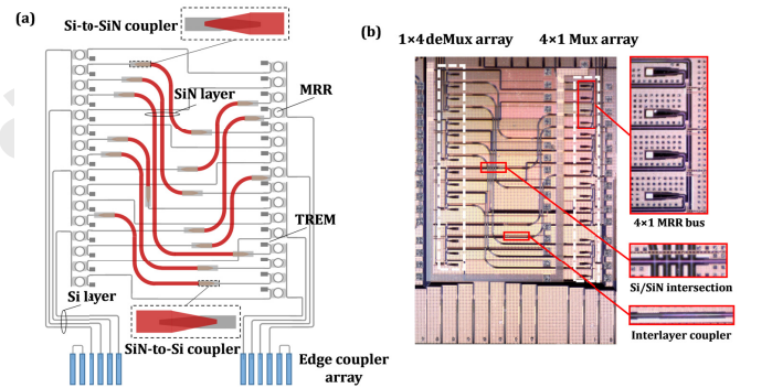
Fig. 3. (a) Schematic layout of the 4 \times 4 MRR-based switch-and-select switching fabric with insets showing the interlayer couplers. (b) Microscope photo of the fabricated device with insets of the enlarged 4 \times 1 MRR-based spatial multiplexer, the Si/SiN intersections and the interlayer coupler.
