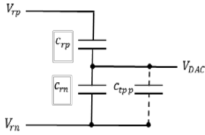
Fig. 4. Equivalent schematic for V_{DAC} generation.
