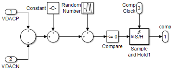
Fig. 6. Fully differential comparator model.
