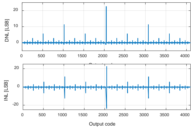
Fig. 9. DNL/INL plot with settling time allocation of 4.5\tau .
