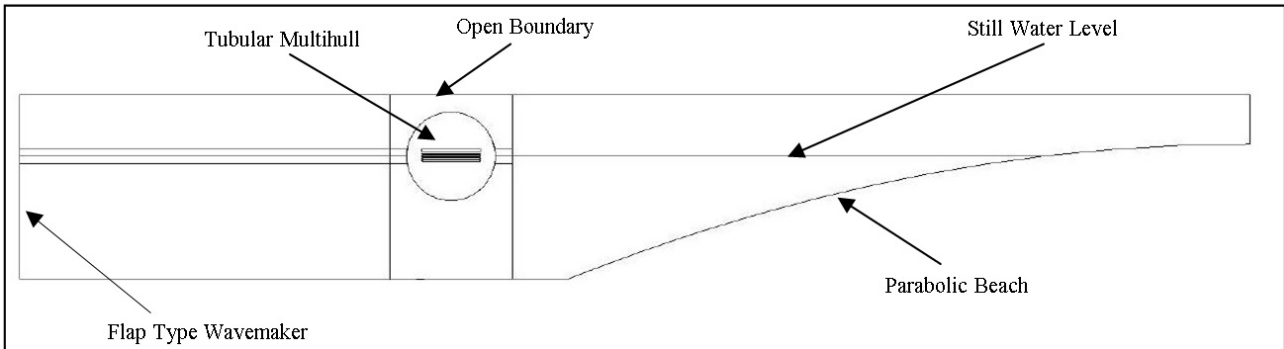
Figure 9: CFD Layout
