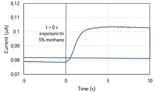
Figure 11. Current response to an exposure of 5% methane
