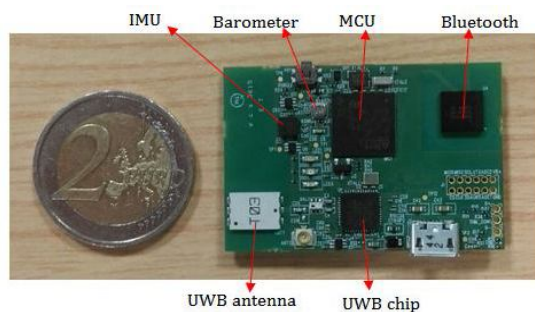
Figure 3. Hybrid Inertial, Positional and Navigation Module
