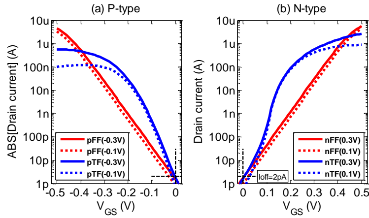
Figure 2: (a) p -type and (b) n -type transfer-characteristics ( I_D - V_{GS} ) at |V_{DS}| = 0.1 V and 0.3 V of single FinFET (FF) and TFET (TF) devices, aligned at I_{off} \sim 2 pA at V_{DD} = 300 mV.
