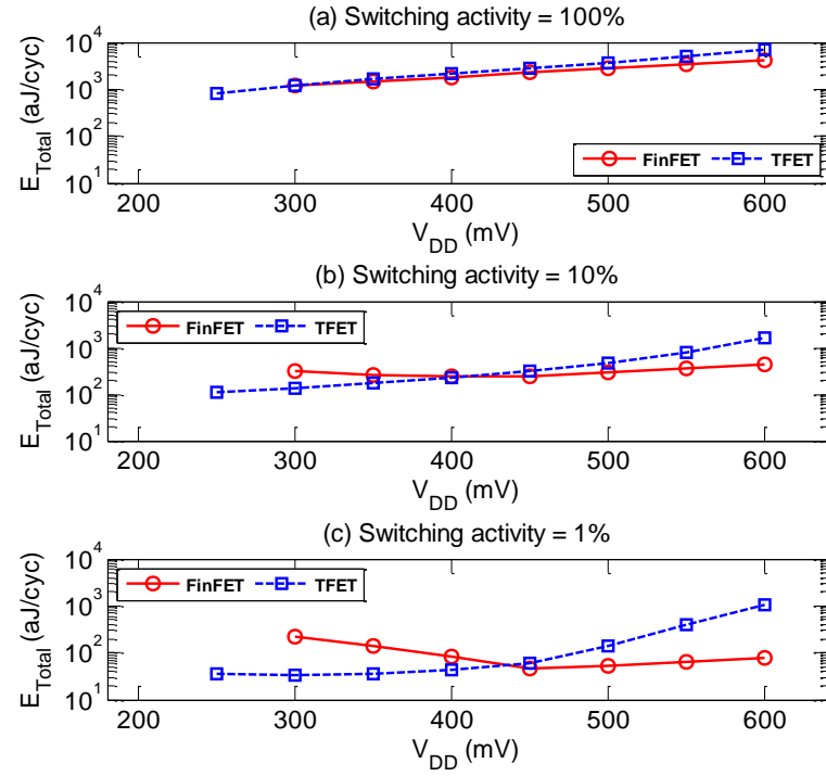
Figure 13: Total Energy (Static + Dynamic contributions) as a function of V_{\text{DD}} for 32-bit Ripple-Carry-Adders, considering a switching activity equal to (a) 100%, (b) 10% and (c) 1%.
