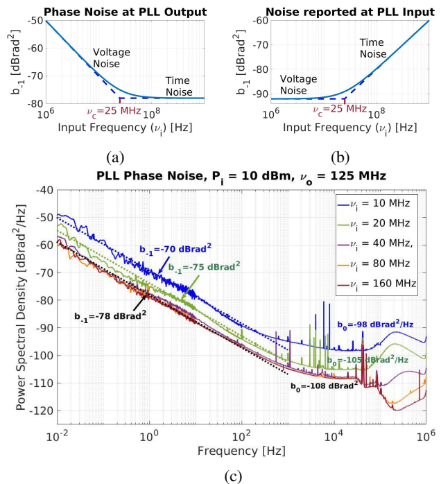
Fig. 5: PLL phase noise. The input slew rate is swept by changing \nu_i in powers of two at a fixed amplitude. a) Behavior of the parameter b_{-1} with respect to the input frequency and reported at the PLL output. b) Canonical form of b_{-1} . Phase noise reported at PLL input. c) Phase noise PSD of PLL output.
