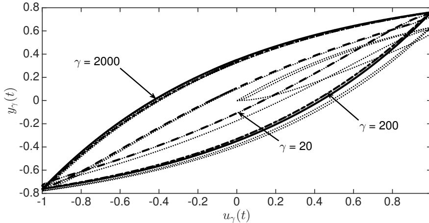
Figure 4: Output of system (15), y_\gamma versus u_\gamma . Dotted: transient; solid: steady state for \gamma = 2000 ; dashed: steady state for \gamma = 200 ; dash-dotted: steady state for \gamma = 20 .
