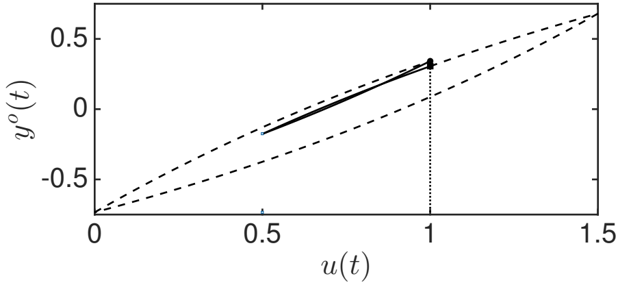
Figure 12: Hysteresis loop G_u^o for \sigma_0 = 1 (minor loop in solid line).
