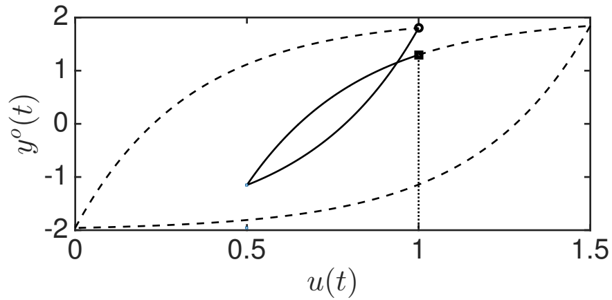
Figure 11: Hysteresis loop G_u^o . The marker open circle corresponds to the point (u(t_1), y^o(t_1)) whilst the marker rectangle corresponds to the point (u(t_5), y^o(t_5)) . The minor loop is plotted in solid line.
