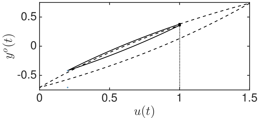
Figure 13: Hysteresis loop G_u^o for \sigma_0 = 1 and u_{\min,2} = 0.2 (minor loop in solid line).
