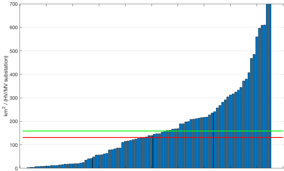
Figure 50. Area per HV/LV substation
