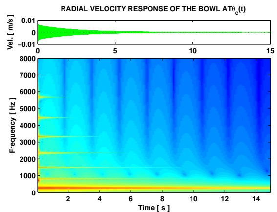
Figure 4: Radial velocity time-history and corresponding spectrogram for external (top) and internal (bottom) rubbing excitation.
