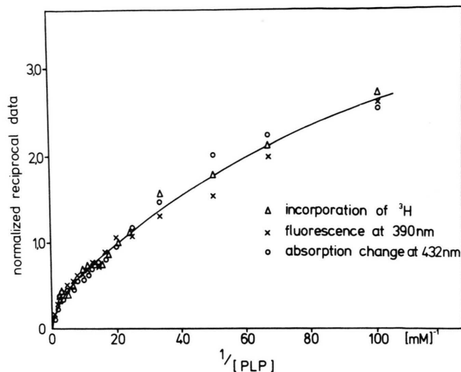
Fig. 1. Double reciprocal diagram for the binding of PLP to the spinach carboxylase a) Absorption change at 432 nm (○); b) fluorescence of the reduced carboxylase-PLP-complex (×) and c) tritium incorporation into the carboxylase-PLP-complex by reduction with NaBT 4 (△) as a function of the reciprocal PLP concentration. All data were normalized on the corresponding result at a PLP concentration of 0.05 mM. Experimental conditions as described under Methods.
