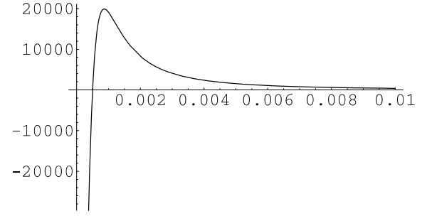
Figure 2. Regularized energy density E(t, x) for \Omega = (0, \infty) and t = 0.001 .
