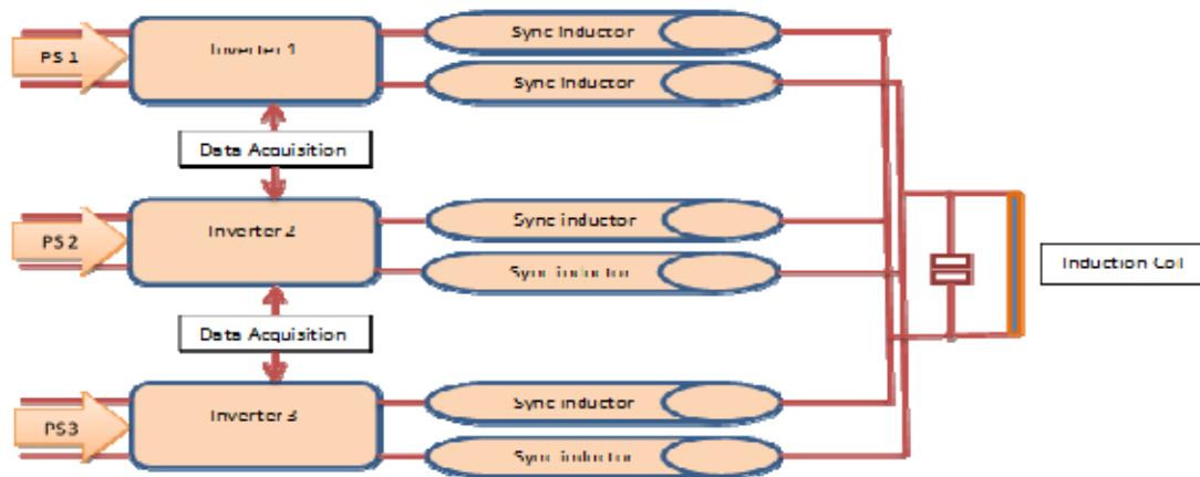
Figure: 02; Induction furnace multiply power source (PS: power source)
