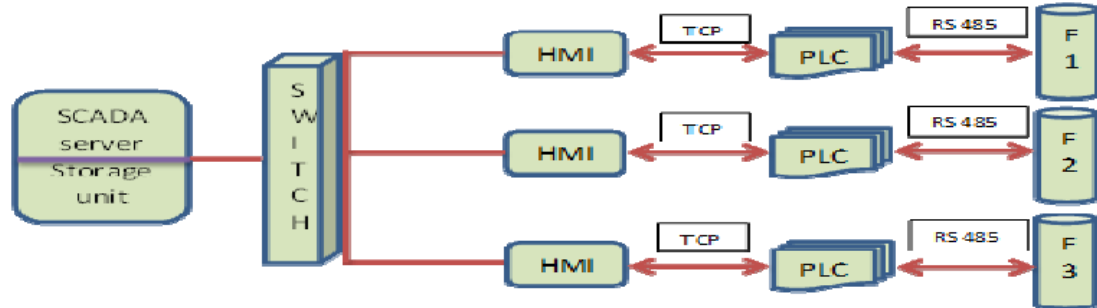
Figure: 04; Hardware design of furnace control.
