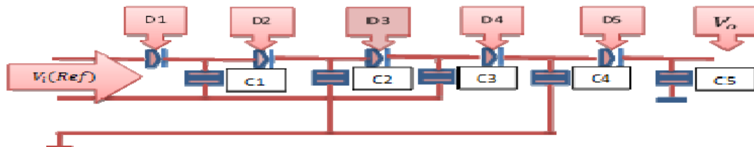
Figure: 6; voltage multiplier diagram
