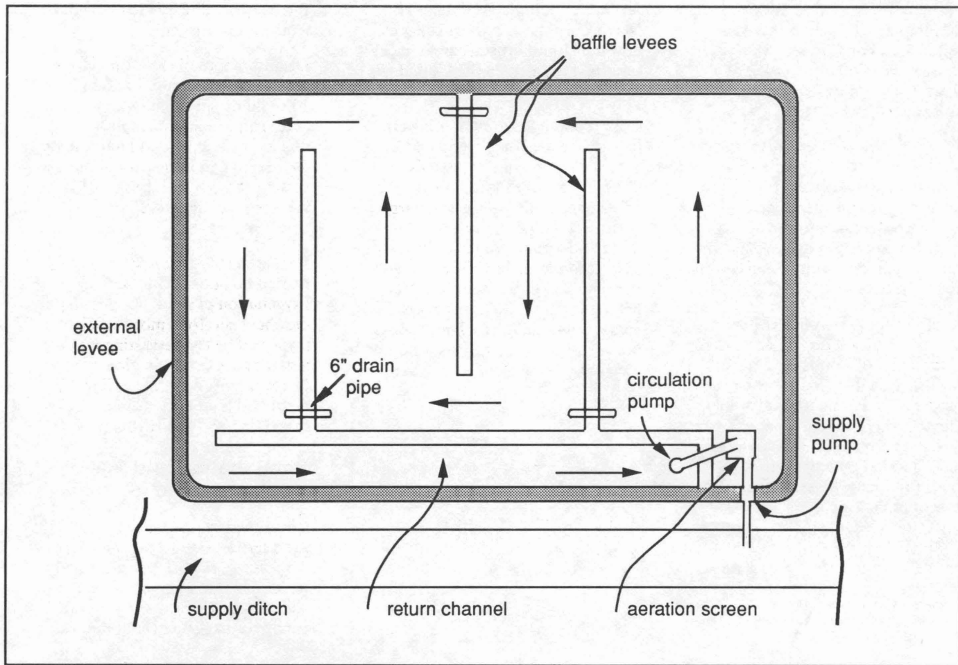
Figure 1. Recirculation design for crawfish pond.
