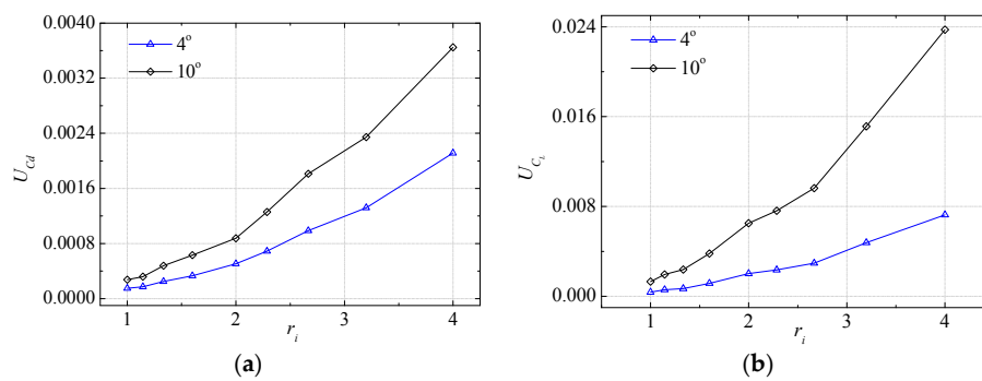
Figure 6. Uncertainty of the drag and lift coefficient with the grid refinement for different attack angles: (a) U_{Cd} ; (b) U_{CL} .
