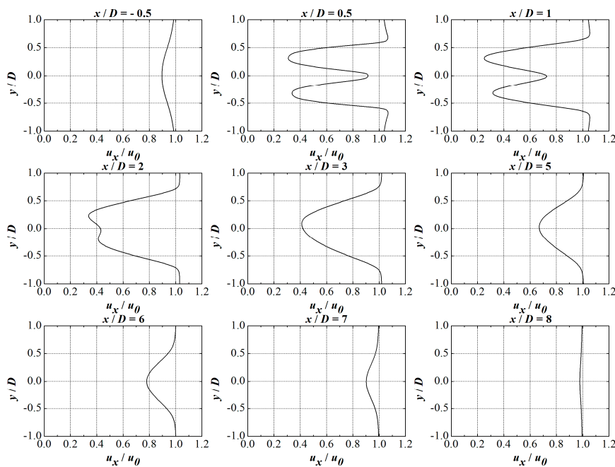
Figure 17. Spanwise distribution of average axial velocity in different streamwise locations.
