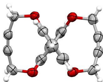
Figure 3. Single-crystal X-ray structure of bis-strained alkyne 3 (ellipsoids plotted at the 50% probability level).
