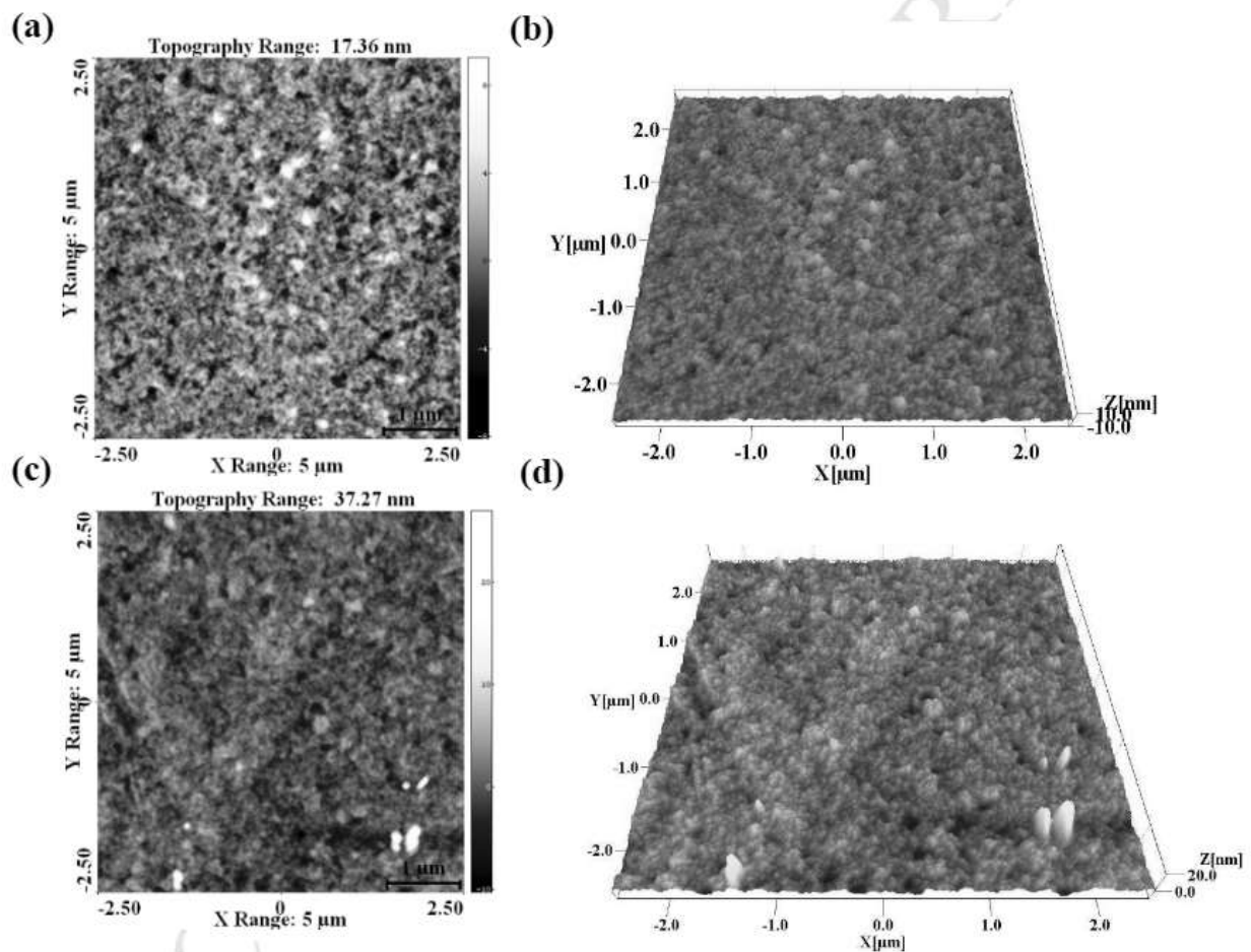
Figure 3: 2D and 3D AFM topography images of GO/PEDOT:PSS films under UVO exposure for (a, b) 0 and (c, d) 10 m treated samples. The AFM scan area is 5\mu\text{m} \times 5\mu\text{m} for GO/PEDOT:PSS films coated on ITO/glass substrates.
