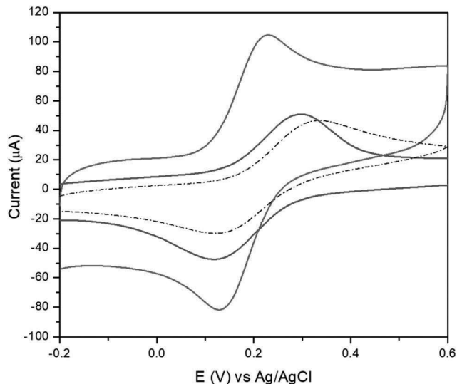
Fig. 1 CVs recorded at the bare GCE (dotted line), TPQPCL 0.025% (blue line), TPQPCL/GNPs 0.025% (red line) containing 5 mM Fe(CN) 6 4- and 0.1 M NaCl supporting electrolyte solutions; scan rate, 100 \text{mV s}^{-1} .
