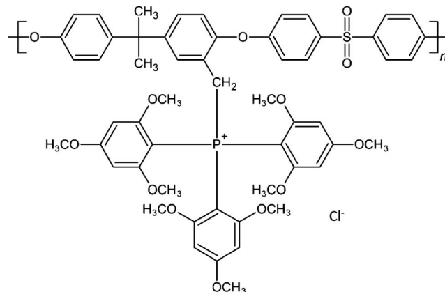
Scheme 1 Structure of tris(2,4,6-trimethoxyphenyl)polysulfone-methylene quaternary phosphonium chloride (TPQPCI).
