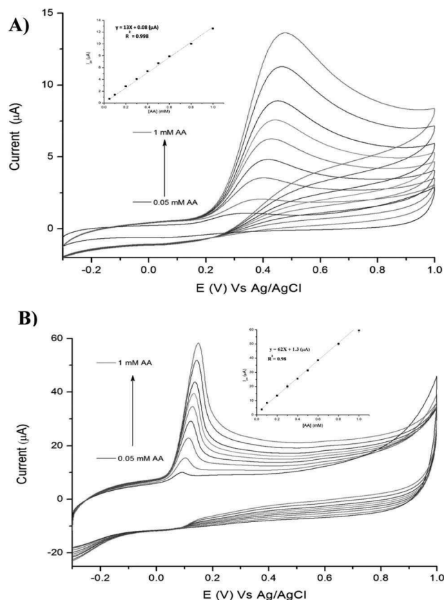
Fig. 5 CVs of (A) TPQPCL and (B) TPQPCL/GNPs at different concentrations of AA from 0.05 mM to 1 mM recorded in the 0.1 M NaCl supporting electrolyte (pH 4); scan rate, 50 \text{mV s}^{-1} . Inset: Plot of anodic peak currents vs. concentration of AA.
