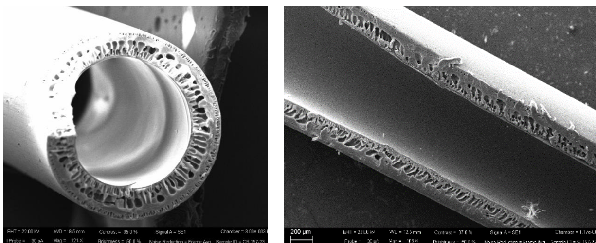
Figure 8. SEM images of the cross section of the porous PAN-based HF.
