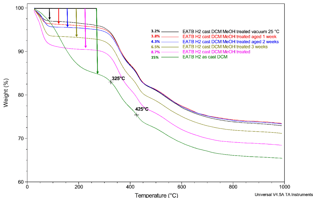
Figure 2. TGA of PIM-EA(H 2 )-TB films. a) Overlay of two films cast from CHCl 3 or DCM; b) overlay of a film cast from DCM, MeOH-treated and aged.
