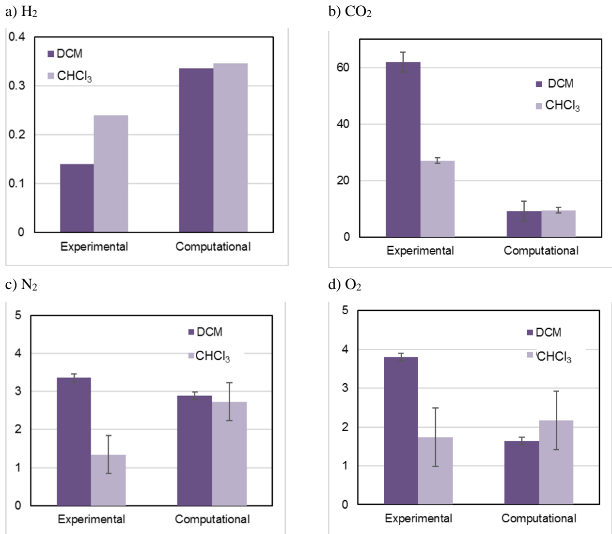
Figure 4. Gas solubility coefficients ( \text{cm}^3 (STP) \text{cm}^{-3} polymer·bar -1 ) in PIM-EA(H 2 )-TB films cast from DCM or CHCl 3 . a) H 2 , b) CO 2 , c) N 2 and d) O 2 . Experimental vs. computational values.
