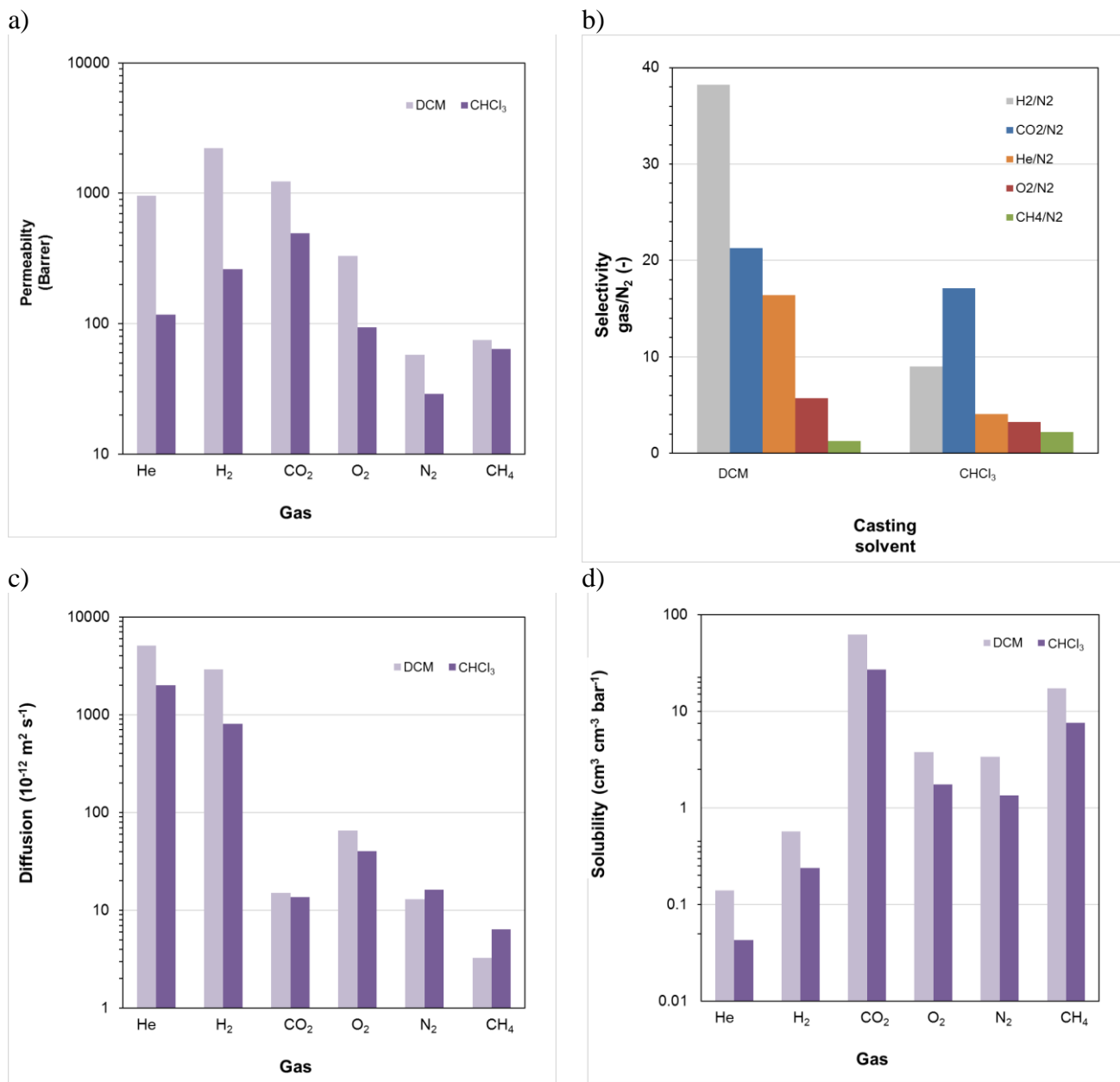
d)Figure 3. Permeability (a), ideal selectivity (b), diffusion (c) and solubility (d) of different gases in films of PIM-EA(H 2 )-TB cast from DCM or CHCl 3 . Gases are in the order of their relative size (kinetic diameter [55]).
