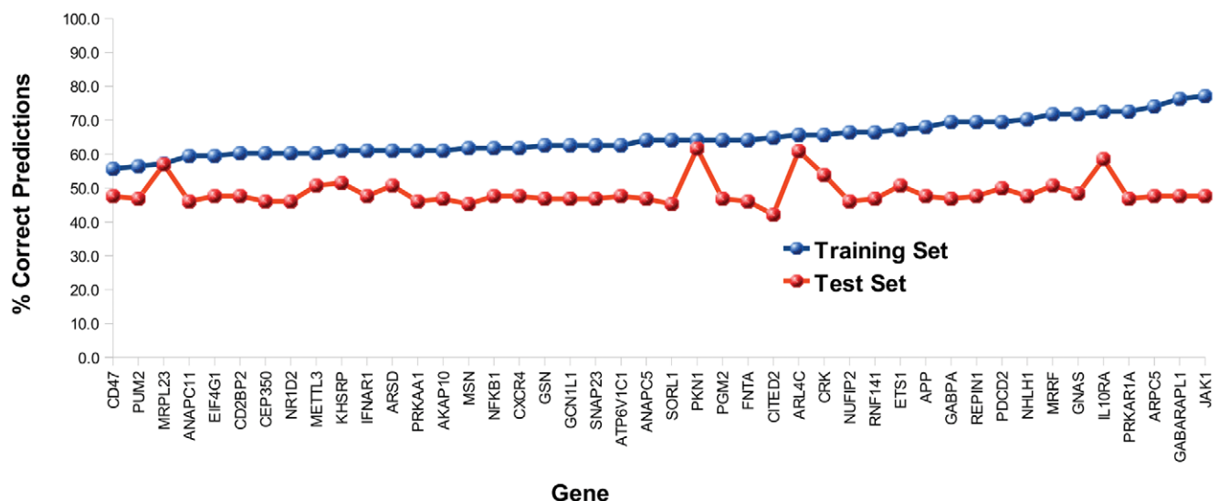
Figure 6. Percentage of predictions made correctly by each of the reporter genes using cut-offs corresponding to a FPR of 5% on the training set (blue) and the test set (red). doi:10.1371/journal.pone.0016872.g006
