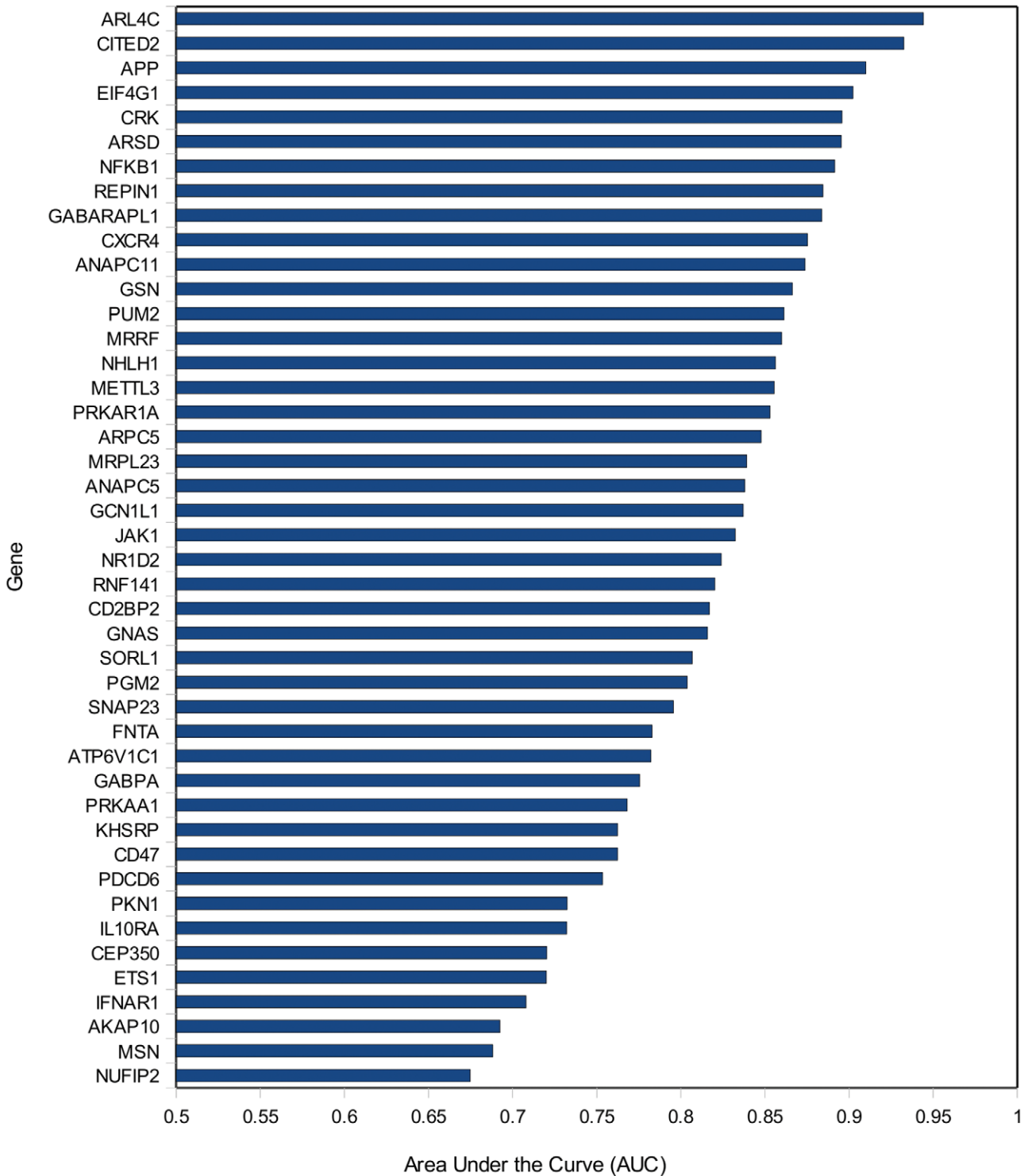
Figure 3. Area under the curve (AUC) values for each of the reporter genes when used as CFS predictors on the training set. All perform better than random (AUC = 0.5). doi:10.1371/journal.pone.0016872.g003
