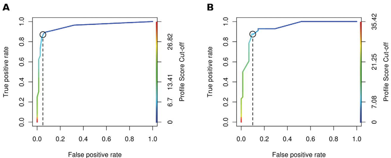
Figure 5. ROC curves for the gene profile score metric using a false positive rate (FPR) on the training set of (A) 5% and (B) 10%. For more detail, see Materials and Methods. The graph is coloured to indicate the gene profile score cut-offs associated with each pair of true and false positive rates at that particular point in the ROC curve. The range of profile cut-off scores are coloured on the right hand y-axes of each graph. The profile score cut-offs used to classify the test set were derived by selecting scores yielding FPR's of (A) 5% and (B) 10%, as indicated by the dashed lines. doi:10.1371/journal.pone.0016872.g005
