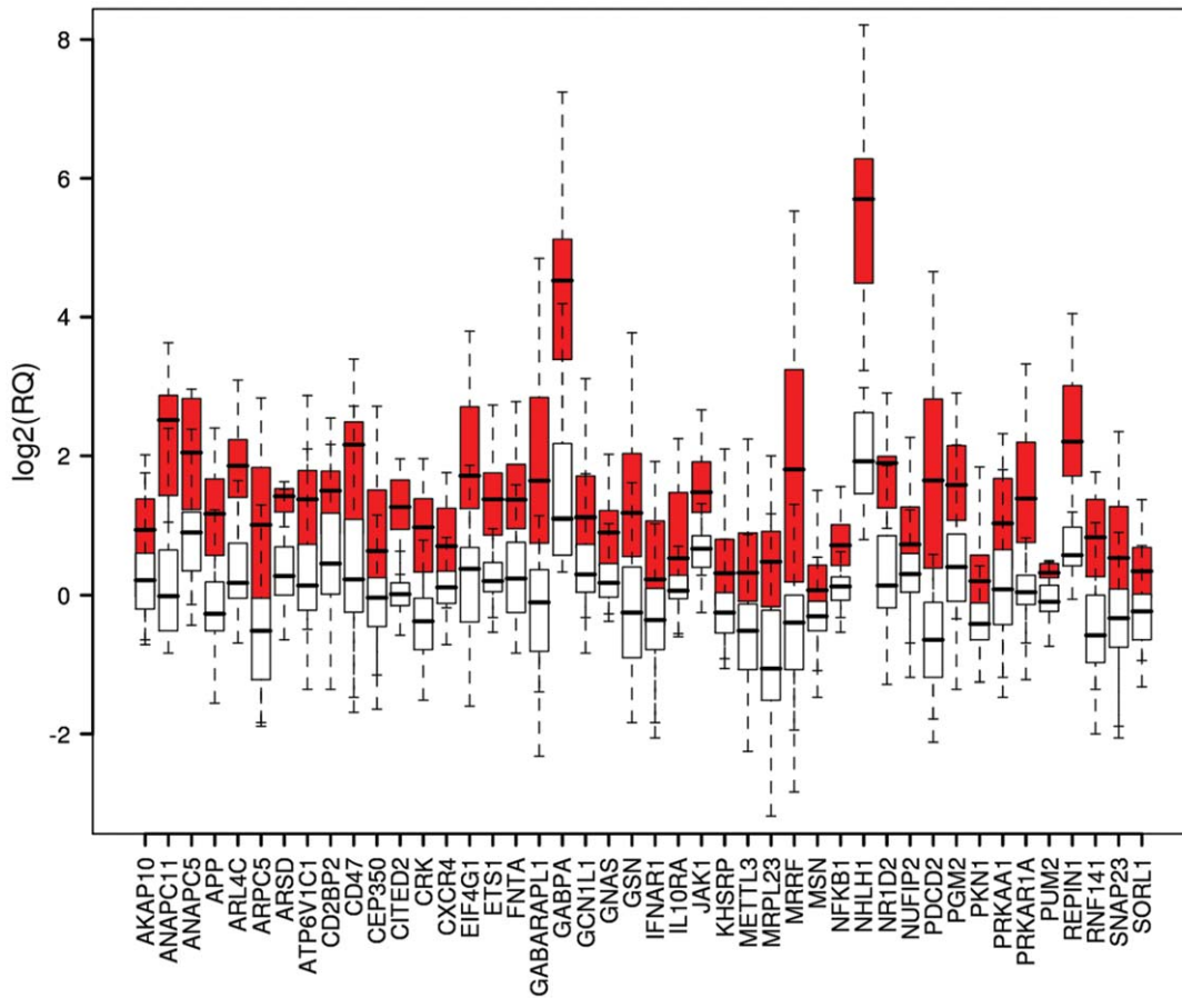
Figure 1. A boxplot illustrating the distribution of \log_2(RQ) values for each of the reporter genes in the training set. Distributions for CFS samples are shown in red, healthy samples in white. The boxes represent the inter-quartile range (25–75%) of the data with the median being shown as a solid horizontal line within each box. Whiskers extend to 1.5 times the inter-quartile range. The data is \log_2 scaled and outliers omitted for purposes of clarity. doi:10.1371/journal.pone.0016872.g001
