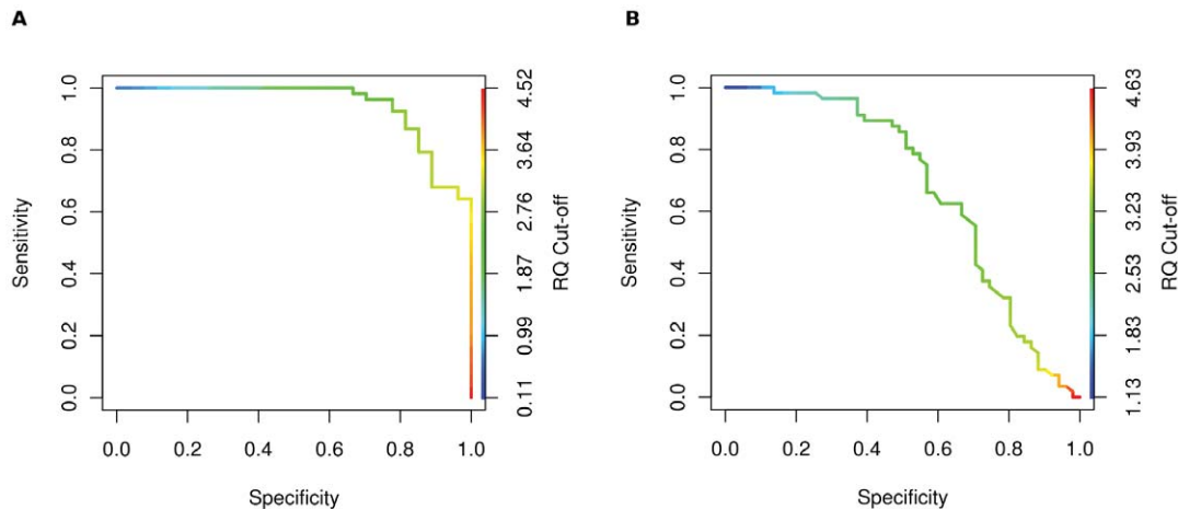
Figure 2. ROC curves obtained when using (A) ARL4C and (B) NUFIP2 as CFS predictors on the training set. The graphs are coloured according to the scale bar on the right hand y-axes to indicate the RQ value cut-offs associated with each pair of sensitivity and specificity values at that particular point in the ROC curve. The AUCs were found to be: (A) 0.94 and (B) 0.67. doi:10.1371/journal.pone.0016872.g002
