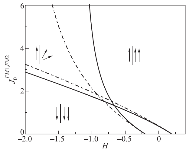
FIG. 5. Regions of collinear, anticollinear, and canted structures in the FM part of the subsystem in a sandwich structure with an ideal and rough FM/AFM interface, and two ideal interfaces.
