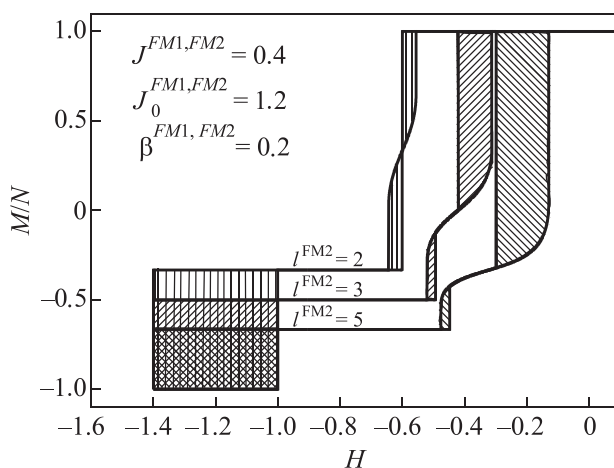
FIG. 7. Magnetization curves for a sandwich FM/AFM/FM system with one ideal and one inhomogeneous FM/AFM interface at varying degrees of inhomogeneity of the FM/AFM interface. Hysteresis regions are marked by hatching. In the bottom hysteresis loop that corresponds to the FM_1 transition, the hysteresis loops for the different degrees of interface inhomogeneity, partially overlap.
