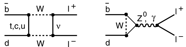
FIG. 1. Representative Feynman diagrams for B^0 \rightarrow \ell^+\ell^- in the standard model.
