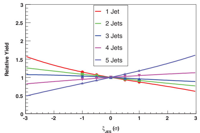
FIG. 1 (color). The function which parametrizes the effect of the jet energy scale on the 1-tag templates of the t\bar{t} sample. Each jet and tag bin for each process in each subsample has a different function for each source of systematic uncertainty. The x axis is in units of the systematic shift.
