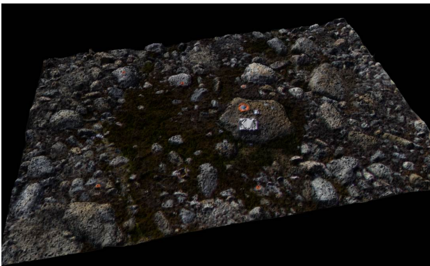
Figure 6: Terrain surface model derived from the point cloud.
