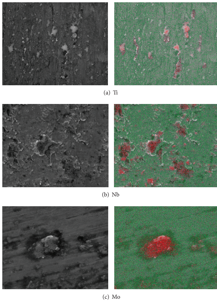
FIGURE 5: FESEM images and corresponding EDS mapping data of Ti (a), Nb (b), and Mo (c) foils heated in liquid Ga.
