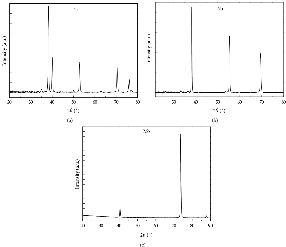
FIGURE 6: XRD peaks of Ti (a), Nb (b), and Mo (c) foils heated in liquid Ga.
