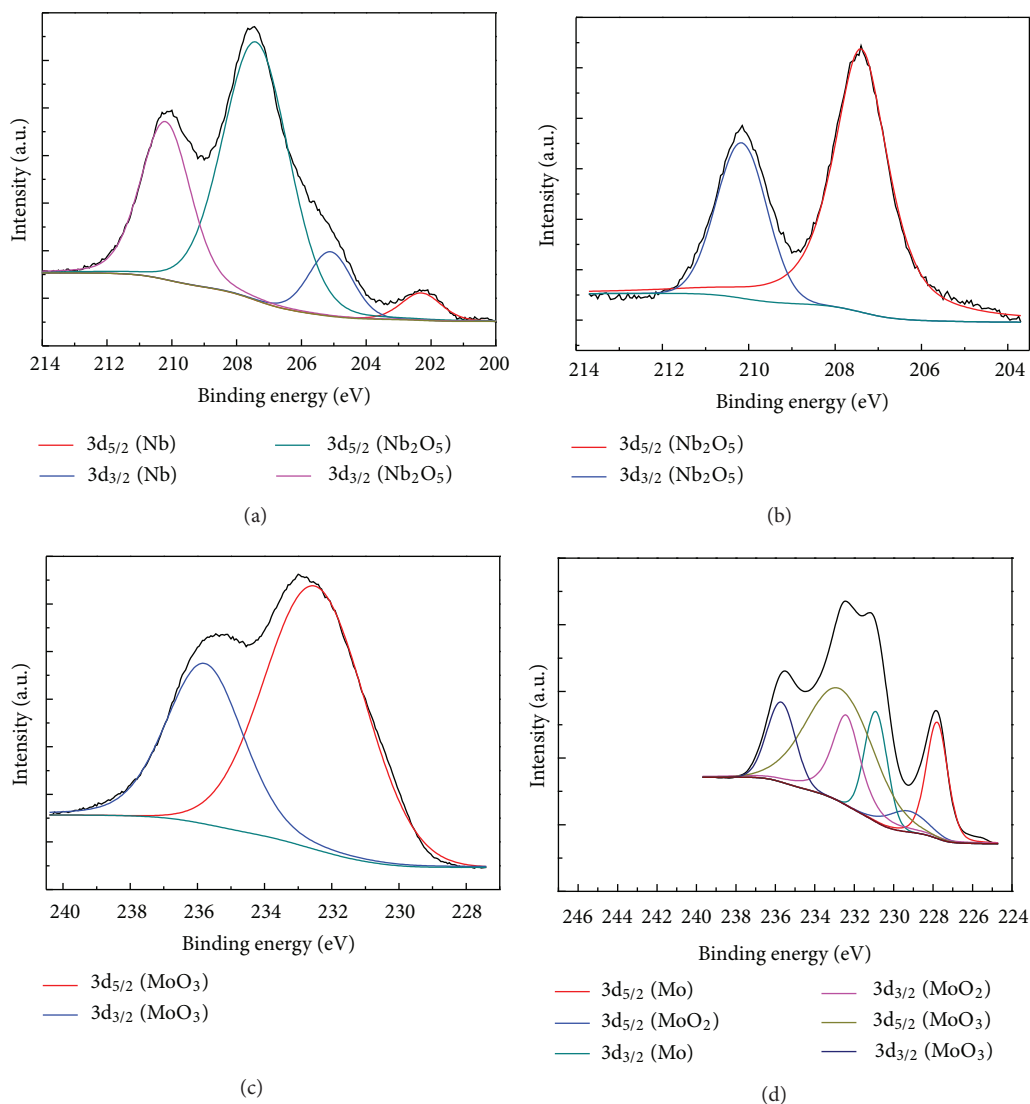
FIGURE 8: 3d peaks of pristine Nb foil (a), Nb foil heated in the liquid Ga (b), pristine Mo foil (c), and Mo foil heated in liquid Ga (d).
