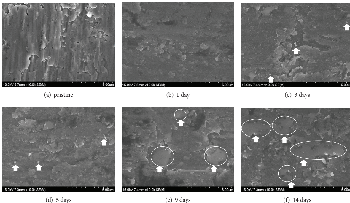
FIGURE 1: FESEM images of pristine Ti foil (a) and Ti foils heated in liquid Ga for 1 day (b), 3 days (c), 5 days (d), 9 days (e), and 14 days (f).
