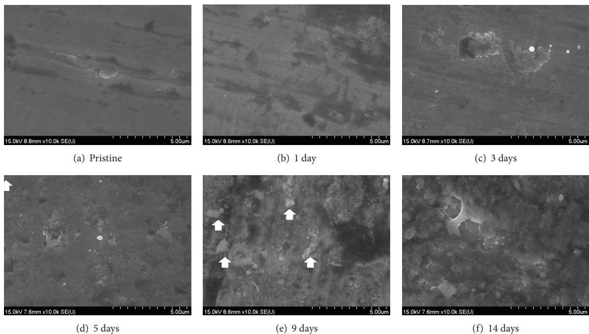
FIGURE 3: FESEM images of pristine Mo foil (a) and Mo foils heated in liquid Ga for 1 day (b), 3 days (c), 5 days (d), 9 days (e), and 14 days (f).
