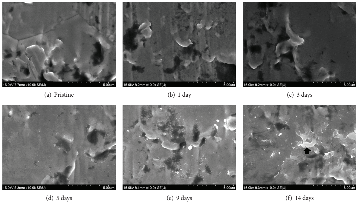
FIGURE 2: FESEM images of pristine Nb foil (a) and Nb foils heated in liquid Ga for 1 day (b), 3 days (c), 5 days (d), 9 days (e), and 14 days (f).
