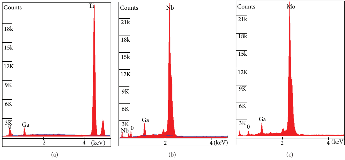
FIGURE 4: EDS peaks of Ti (a), Nb (b), and Mo (c) foils heated in the liquid Ga.
