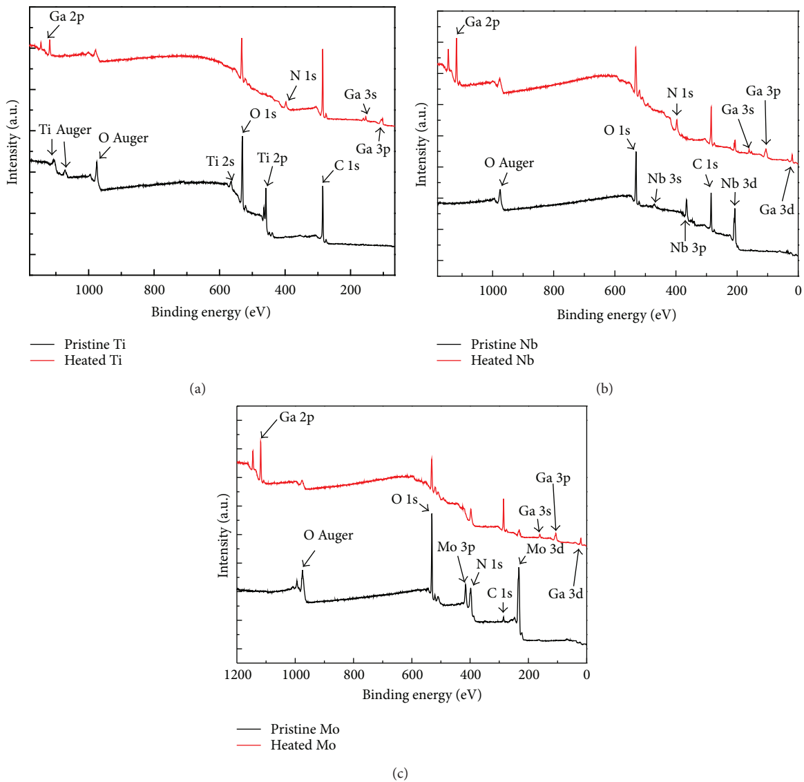
FIGURE 7: XPS survey spectra of Ti (a), Nb (b), and Mo (c) foils before and after heating in the liquid Ga.
