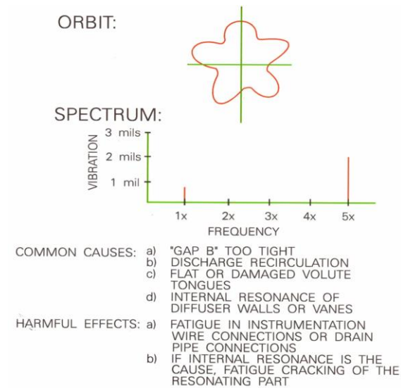
Figure 12. Vane Pass Vibration
