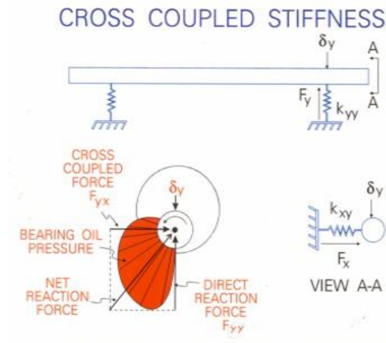
Figure 10. Cross-Coupled Stiffness, a Key Factor in Subsynchronous Whirl & Whip
