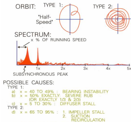
Figure 9. Subynchronous Vibration
