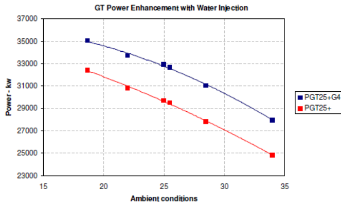
Figure 33. Power Uprate with the New G4 Engine Variant.
