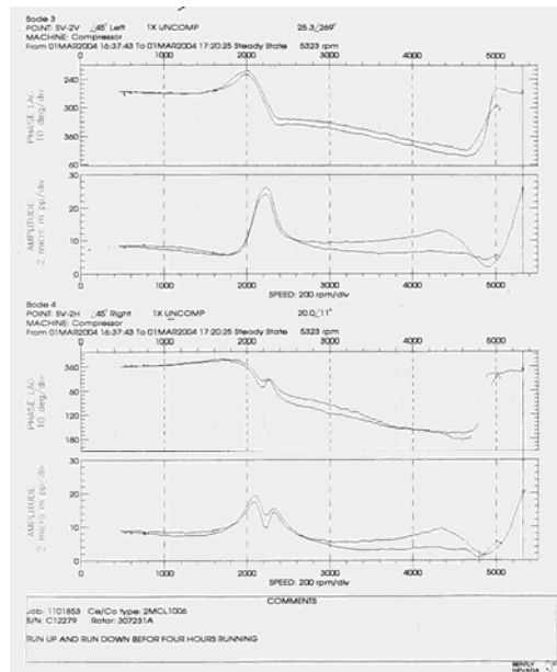
Figure 26. Ethylene Rotor Bode plot Showing Growth in Amplitude and Phase Shift when Operating at MCS.
