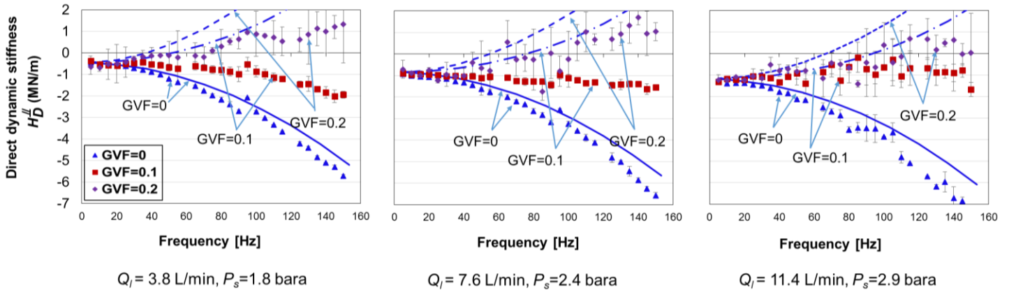
Fig. 24 Upstream step clearance seal: direct dynamic stiffness versus frequency. Inlet GVF = 0, 0.1 and 0.2. Supply oil flow rate Q_l = 3.8 L/min to 11.4 L/min.. Lines: prediction; Symbols: test data.
