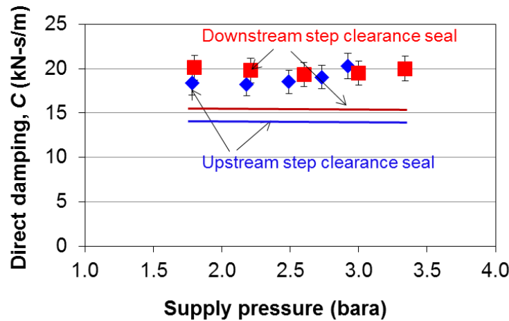
Fig. 23 Direct damping ( C ) versus supply pressure for upstream and downstream step clearance seals. All liquid. Stationary shaft. Lines: prediction; Symbols: test data.
