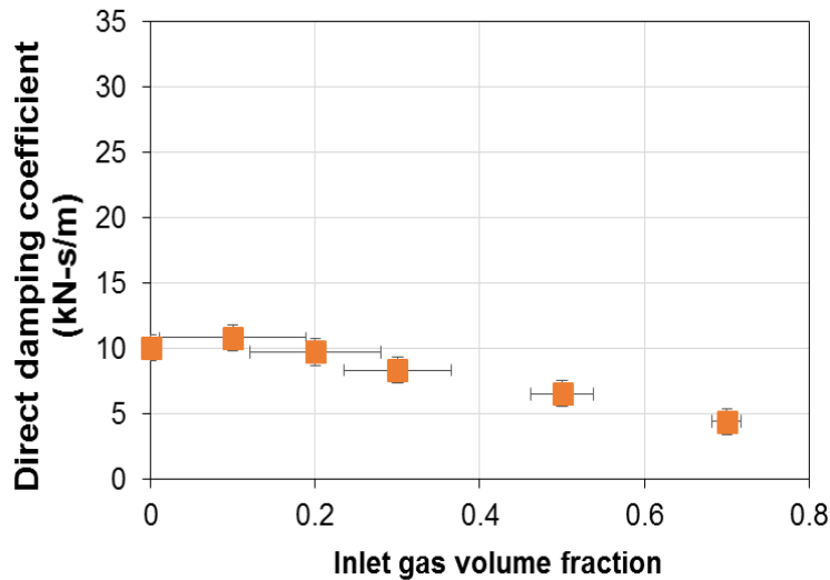
Fig. 18 Grooved seal: direct damping coefficient versus inlet gas volume fraction. Inlet GVF = 0 to 0.7. Shaft speed = 3.5 krpm ( \Omega R = 23.3 m/s). Supply pressure ( P_s ) = 2.9 bara, discharge pressure ( P_a ) = 1 bara.
