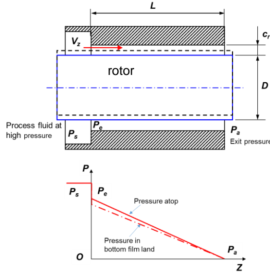
Fig. 2 Geometry of an annular seal and its pressure profile showing a sudden pressure drop at the seal entrance [6].
