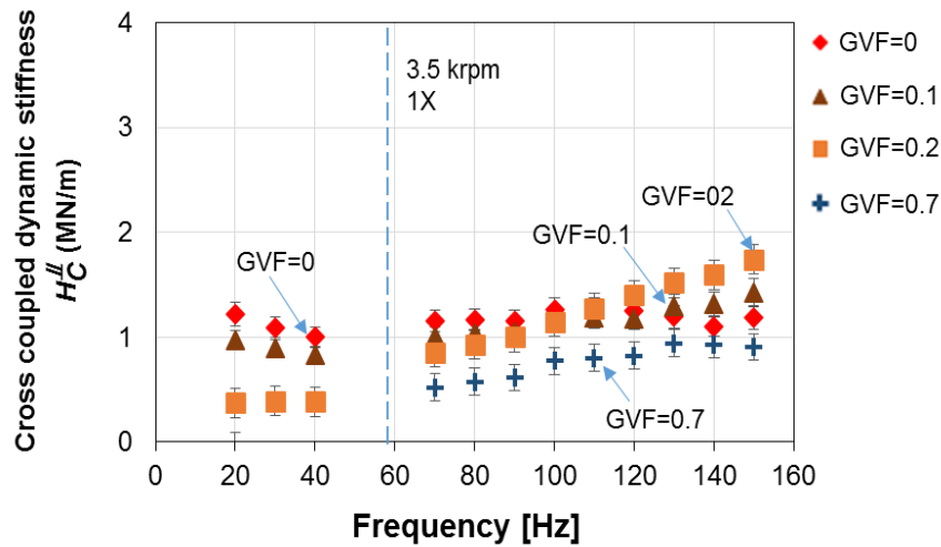
Fig. 17 Grooved seal: cross coupled dynamic stiffness versus frequency. Inlet GVF = 0, 0.1, 0.2, 0.7. Shaft speed = 3.5 krpm ( \Omega R = 23.3 m/s). Supply pressure ( P_s ) = 2.9 bara, discharge pressure ( P_a ) = 1 bara.
