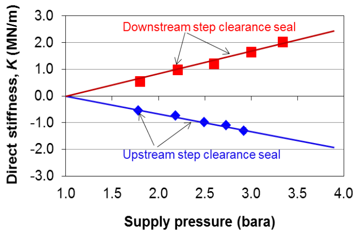
Fig. 21 Static stiffness ( K ) versus supply pressure for upstream and downstream step clearance seals. All liquid. Stationary shaft. Lines: prediction; Symbols: test data.
