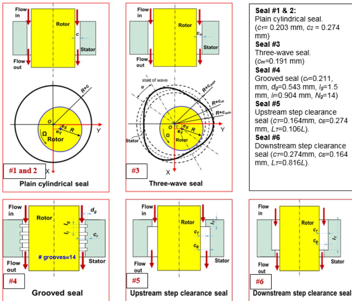
Fig. 6 Schematic views of six test seals: plain, grooved, stepped, and wavy configurations. Clearances exaggerated to illustrate the seal geometries.
