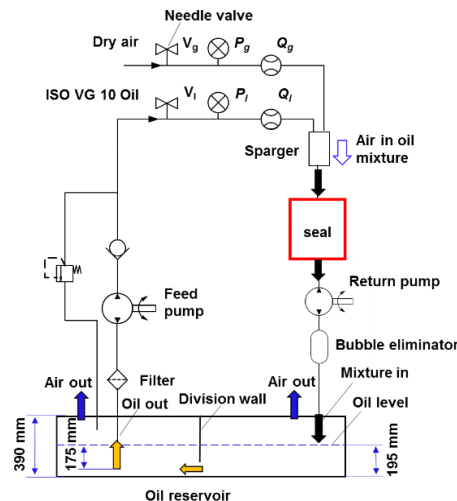
Fig. 5 Air and lubricant circulation flow systems.
