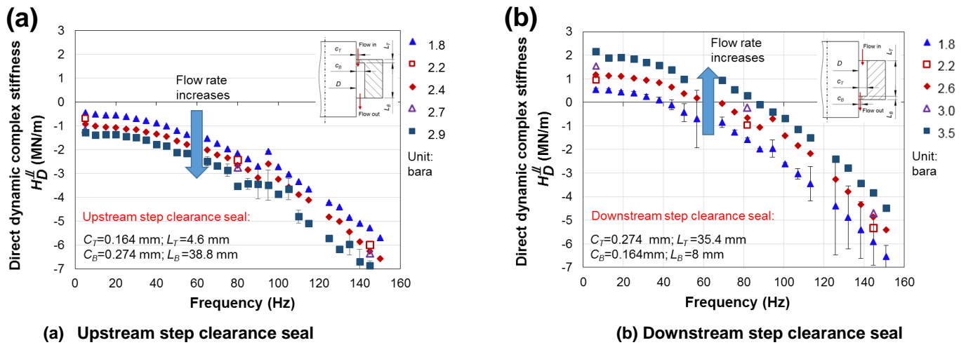
Fig. 20 Direct dynamic stiffness versus frequency for two step clearance seals. Shaft speed = 0 rpm. Supply pressure ( P_s ) = 1.8 to 3.5 bara, discharge pressure ( P_a ) = 1 bara.
