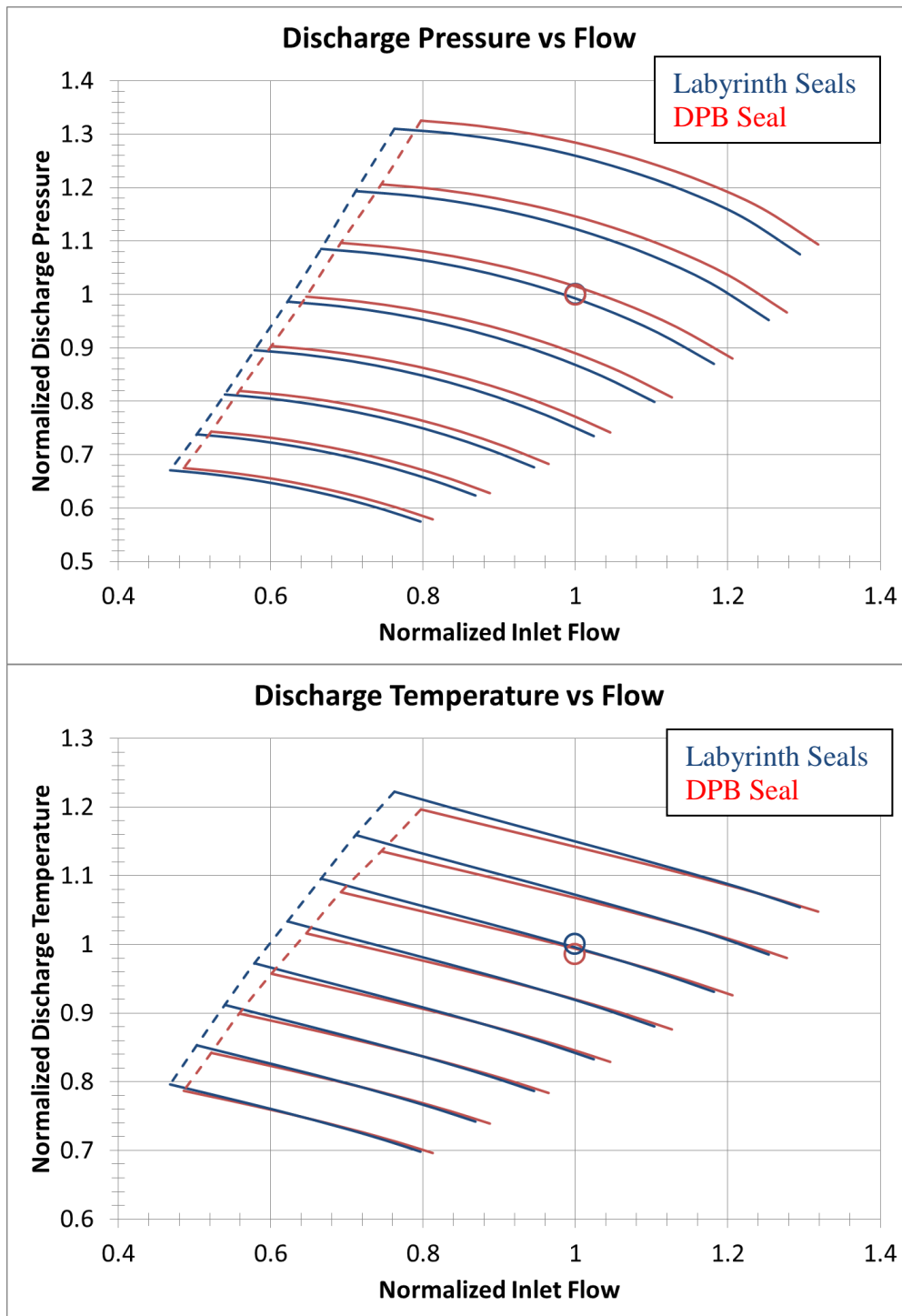
Figure 9: Discharge pressure and discharge temperature versus inlet volumetric flow, flange to flange, both sections.
