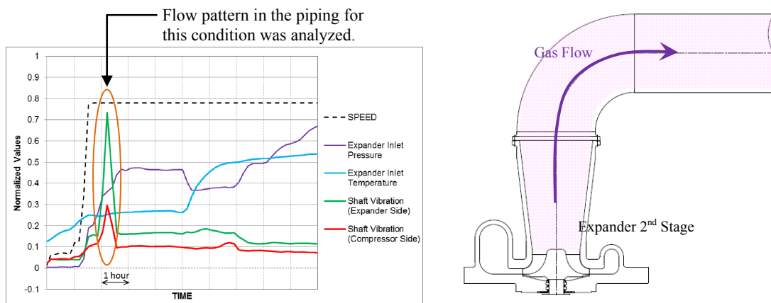
Fig.4 Condition and Objects for CFD Analysis for 2 nd Stage Expander Wheel
