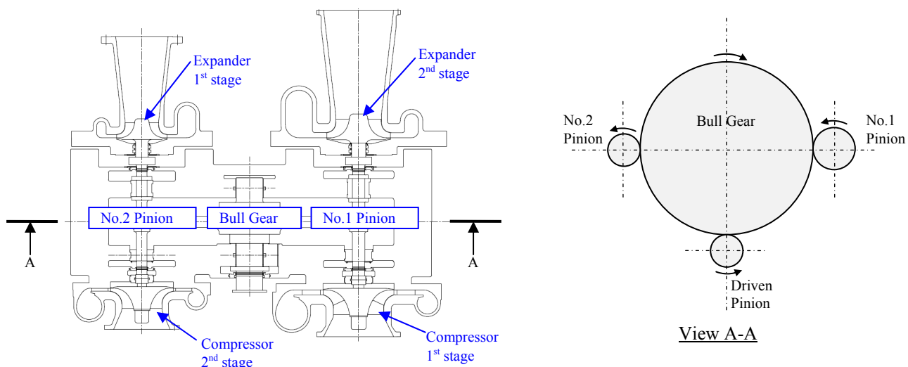
Fig.1 Integally Geared Compressor-Expander
