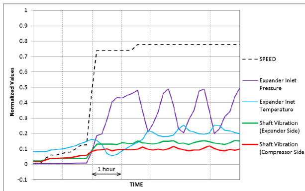
Fig.15 Time Trend Data of Operating Speed, Inlet Pressure/Temperature of Expander 2 nd Stage and Shaft Vibration after Countermeasure
