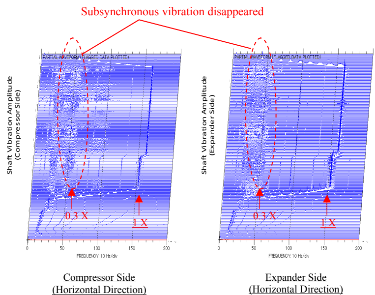
Fig.16 Waterfall Plot of No.1 Pinion Rotor after Countermeasure
