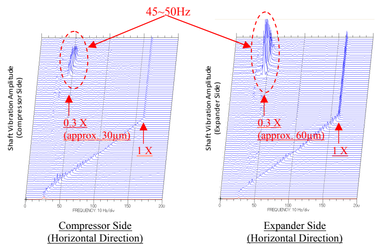
Fig.3 Waterfall Plot during Plant Start Up of No.1 Pinion Rotor
