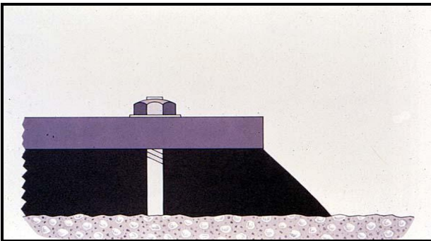
Figure 17: Precision Grout Shoulder with a 45° Chamfer
