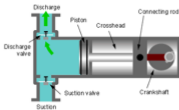
Figure 14: Piston Pump
