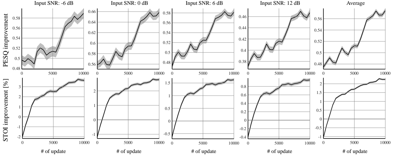
Fig. 5. OSQA score improvement depending on number of updates. X-axis shows number of updates, and y-axis shows average difference between OSQA score of proposed method and that of observed signal. Solid lines and gray area are average and standard-error, respectively.
