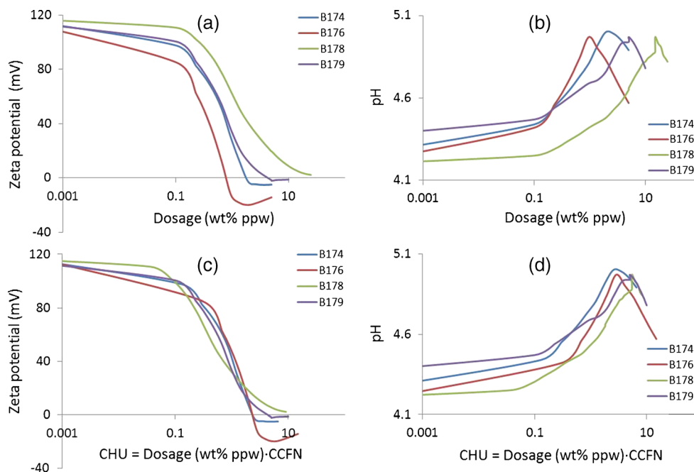
Fig. 3 Evolution of zeta potential and pH of the Al 2 O 3 dispersions during titration with the four dispersants. a Zeta and b pH as a function of dispersant dosage. c Zeta and d pH as a function of CHU (dispersant dosage normalized by CCFN)
