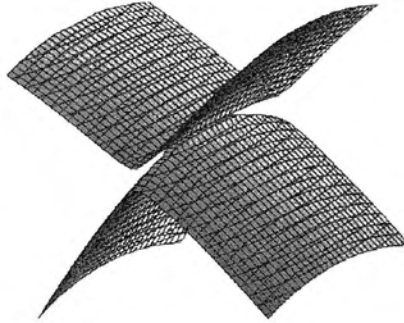
Figure 5: The biplanar double point at the origin of the surface defined by the equation z^2 - (1/2)x^2 + 2yz^2 - 2zx^2 + x^4 + 2x^2y^2 + (1/2)y^4 = 0 .
