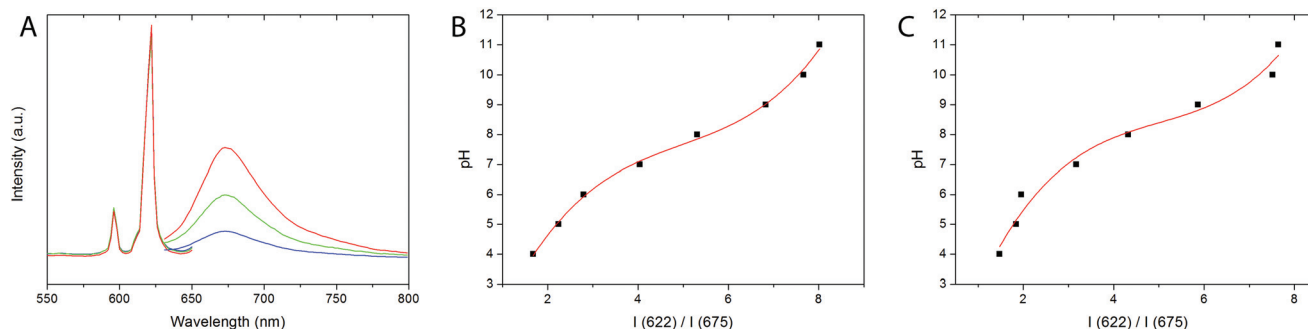
Fig. 9 (A) Emission spectra of the Bi20YPAA2 nanoparticles functionalized with Nile Blue (NB) at pH 5 (red), 7 (green), and 10 (blue). Emission of \text{Eu}^{3+} (left part) was collected with excitation at \lambda_{\text{ex}} = 342 nm, while \lambda_{\text{ex}} for NB was 600 nm (emission on the right part). (B) Intensity ratio of the \text{Eu}^{3+} ( \lambda_{\text{em}} = 622 nm, \lambda_{\text{ex}} = 342 nm) and the NB ( \lambda_{\text{em}} = 675 nm, \lambda_{\text{ex}} = 600 nm) emission at different pH values for the Bi20YPAA2-NB nanoparticles, and Bi20GdPAA-NB particles (C). In both last cases, the error bars are smaller than the size of the symbols.
