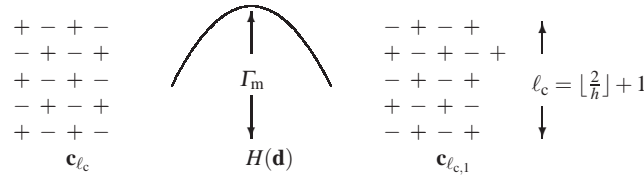
Fig. 7 Graphical description of \Gamma_m for the nearest neighbor PCA.
