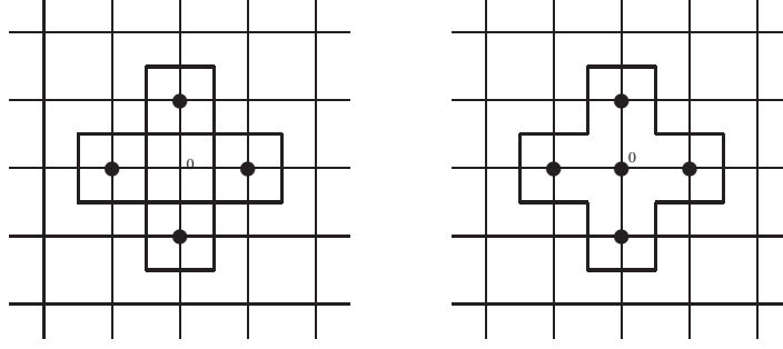
Fig. 2 Schematic representation of the nearest neighbor (left) and cross (right) models.
