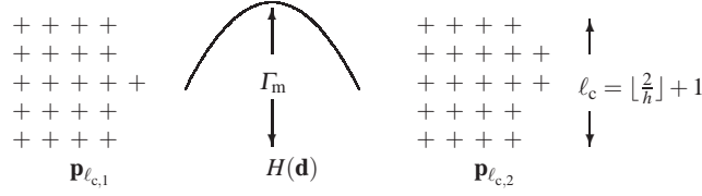
Fig. 6 Graphical description of \Gamma_m for the cross PCA.
