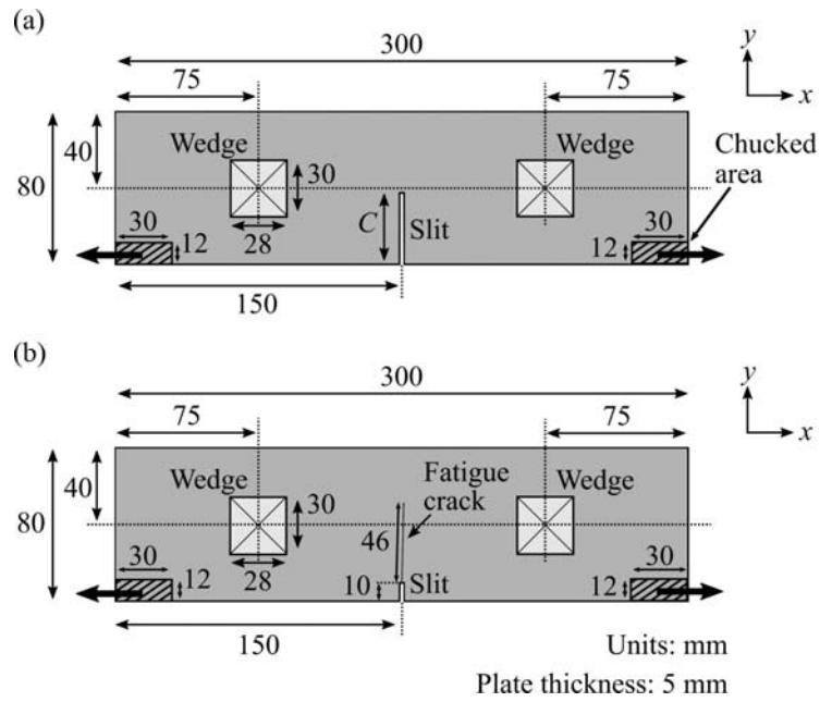
Fig. 5 Schematic of the aluminum alloy plate specimens used in the experiment, (a) specimen with an EDM slit of different lengths C , (b) specimen with a fatigue crack grown from an EDM slit.
