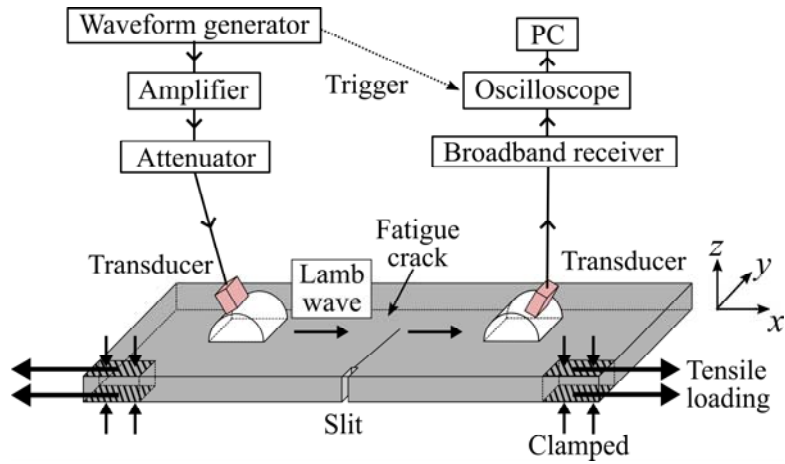
Fig. 6 Schematic of the experimental setup.
